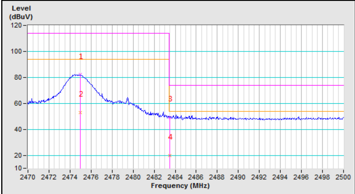
2475MHz Vertical
