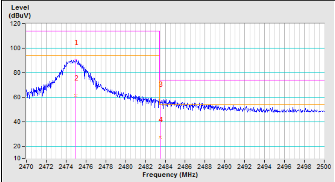
2475MHz Vertical
