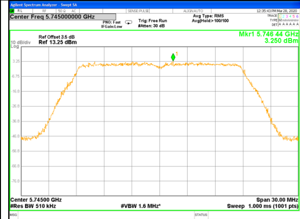
W58_11ax20_Higher_Power Spectrum Density
