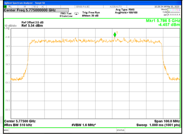
W58_11ax80_Power Density_5775M
