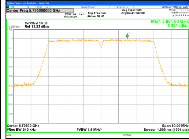
W58_11ax40_Higher_Power Spectrum Density
