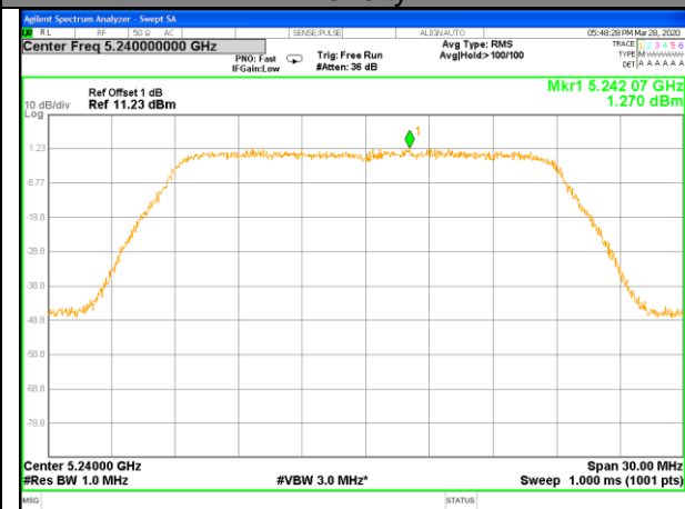
W52_11ax20_Higher_Power Spectrum Density
