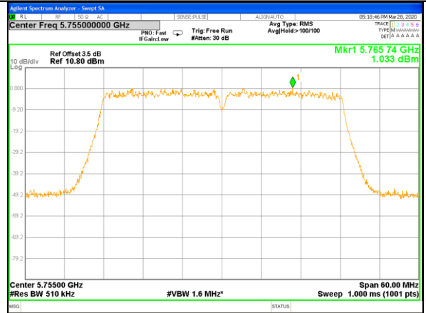
W58_11ax40_Lower_Power Spectrum Density
