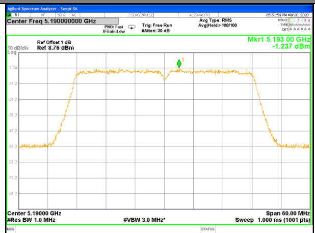
W52_11ax40_Lower_Power Spectrum Density
