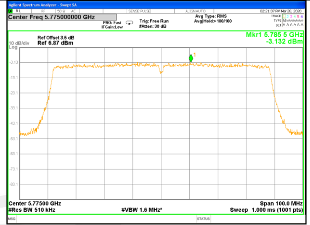
W58_11ax80_Power Density_5775M
