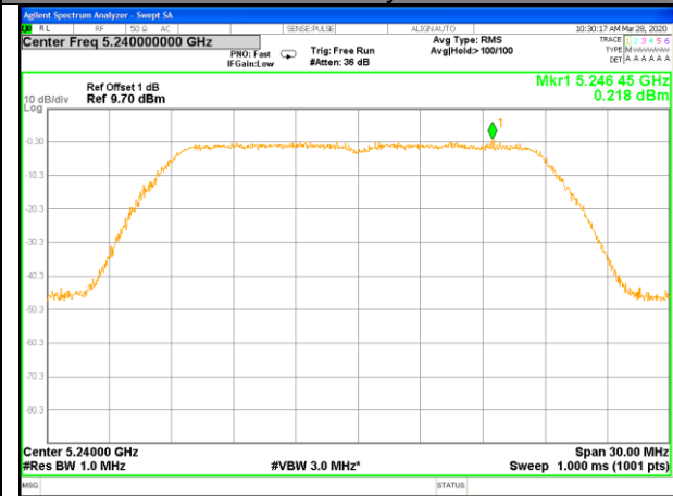
W52_11ax20_Higher_Power Spectrum Density
