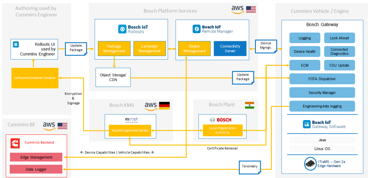
Figure 2: Data Flow diagram with DM and FOTA usecase
