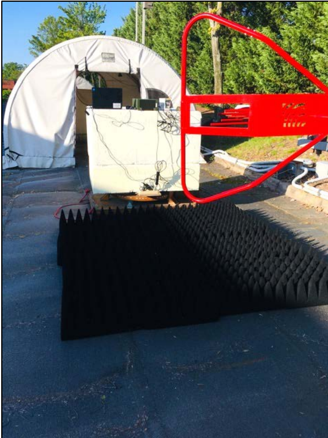
Photograph 4: Radiated Emissions (Spurious/Harmonics) – Back View, Greater than 1 GHz
