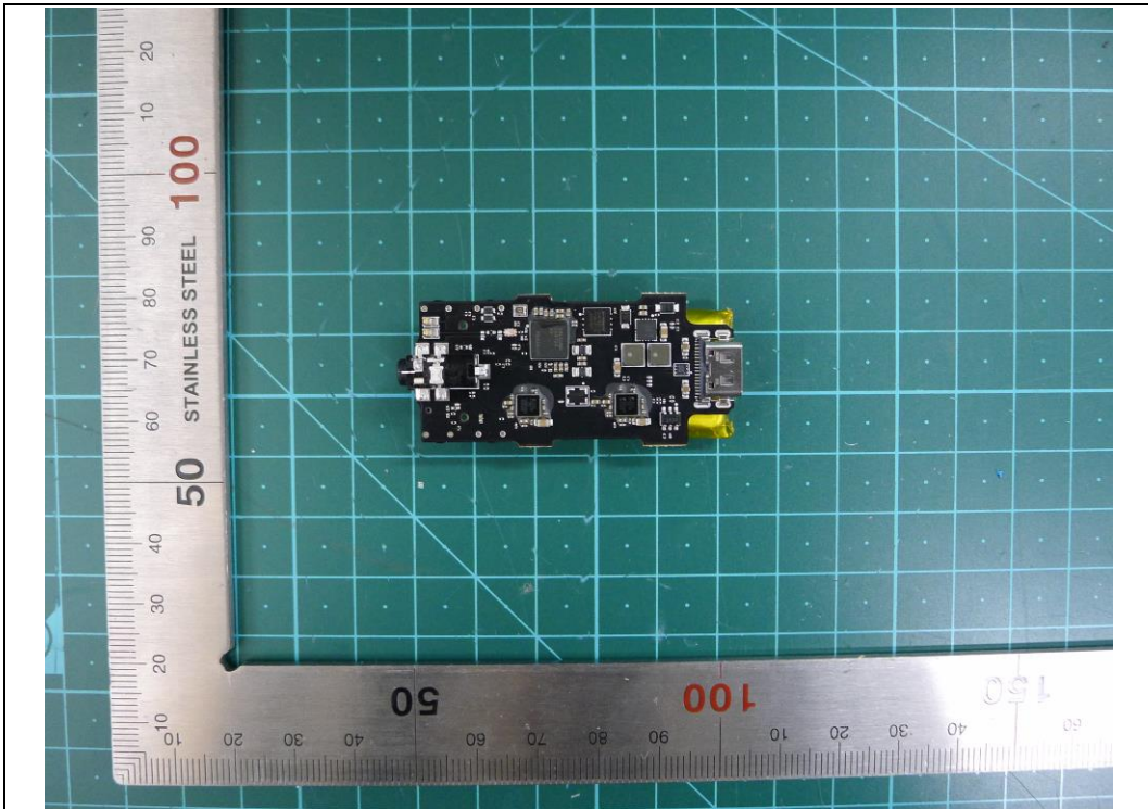
PCB Front
