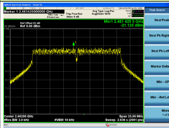
Channel 11 (2462MHz)
