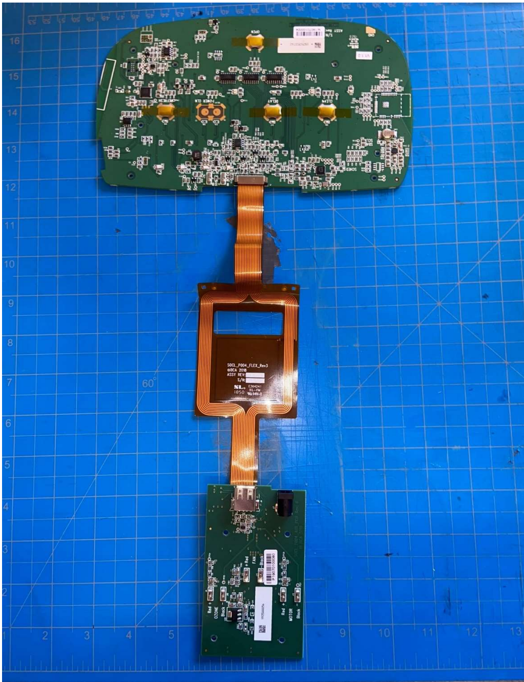
Main Board connected to Auxiliary Board
