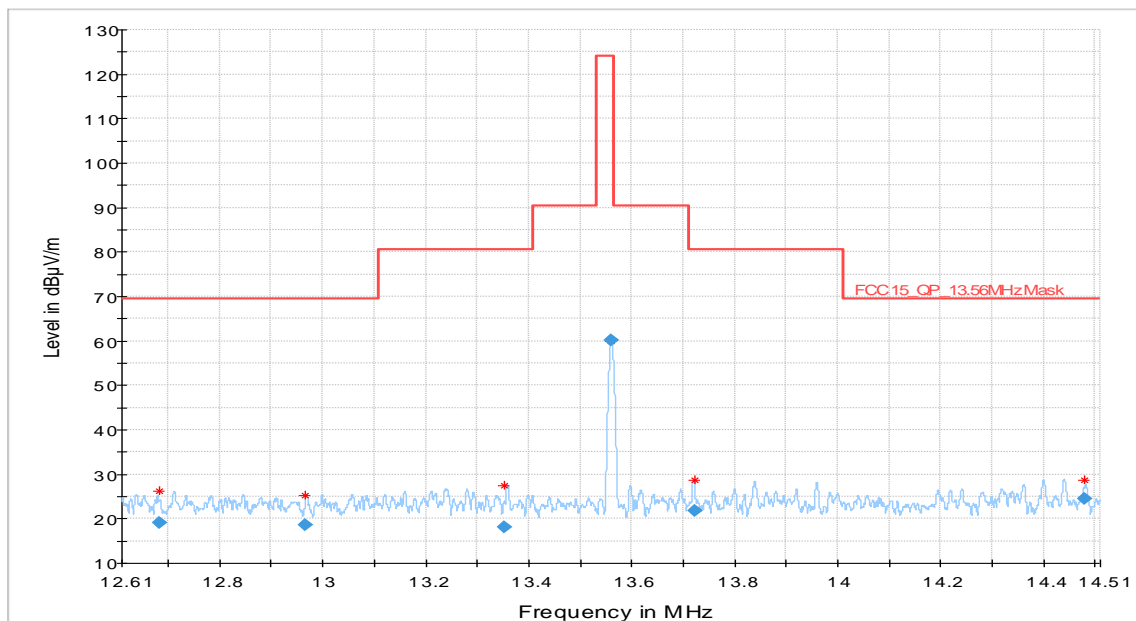
Figure 4: Out of Band Spectrum Mask for RFID Reader – 90 Degree Loop Antenna X-axis
