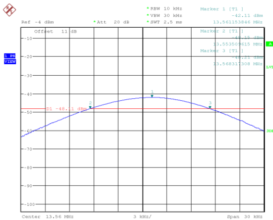
Figure 31: Frequency Stability at 40 °C – 5 min
