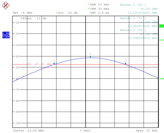
Figure 37: Voltage Variation at 102 VAC
