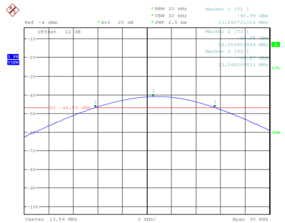
Figure 16: Frequency Stability at 0 °C - 10 min
