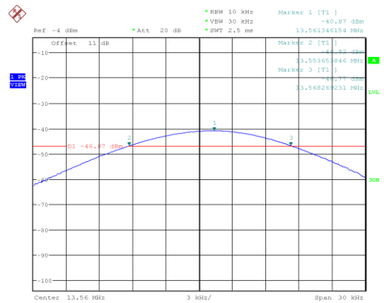
Figure 12: Frequency Stability at -10 °C – 10 min
