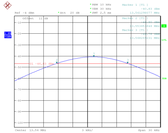
Figure 10: Frequency Stability at -10 °C – 2 min
