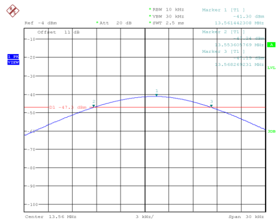
Figure 28: Frequency Stability at 30 °C – 10 min
