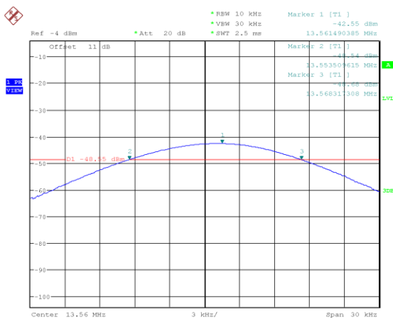
Figure 35: Frequency Stability at 50 °C - 5 min
