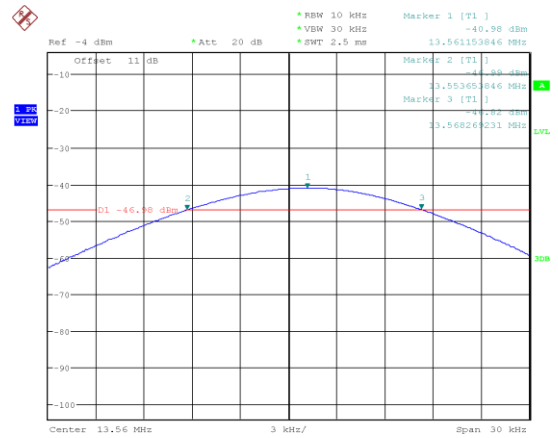
Figure 14: Frequency Stability at 0 °C - 2 min
