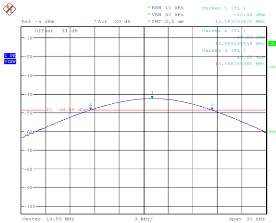
Figure 33: Frequency Stability at 50 °C - Start
