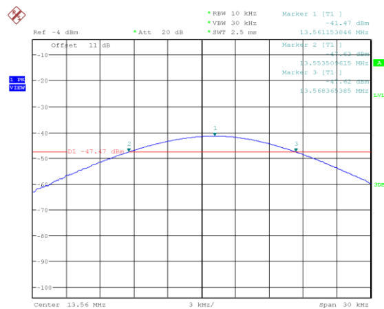
Figure 27: Frequency Stability at 30 °C – 5 min
