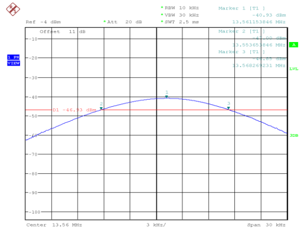
Figure 6: Frequency Stability at -20 °C – 2 min
