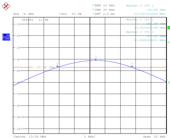
Figure 23: Frequency Stability at 20 °C – 5 min
