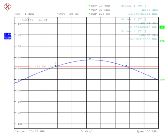
Figure 36: Frequency Stability at 50 °C - 10 min
