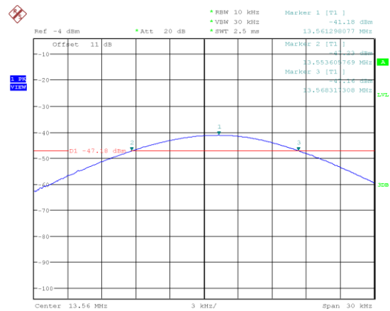
Figure 20: Frequency Stability at 10 °C – 10 min
