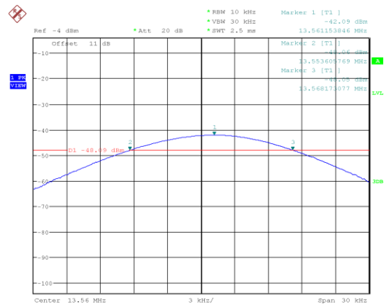
Figure 32: Frequency Stability at 40 °C – 10 min
