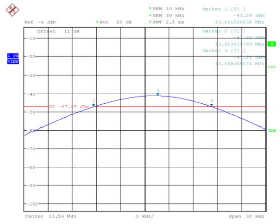
Figure 24: Frequency Stability at 20 °C – 10 min
