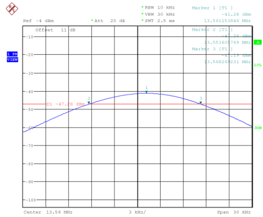
Figure 22: Frequency Stability at 20 °C – 2 min
