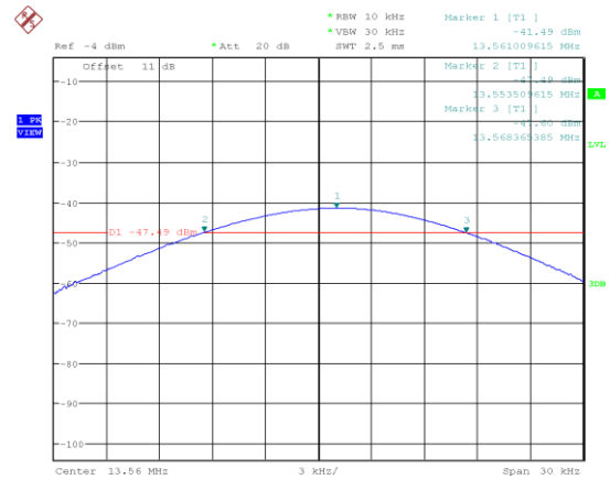
Figure 38: Voltage Variation at 120 VAC
