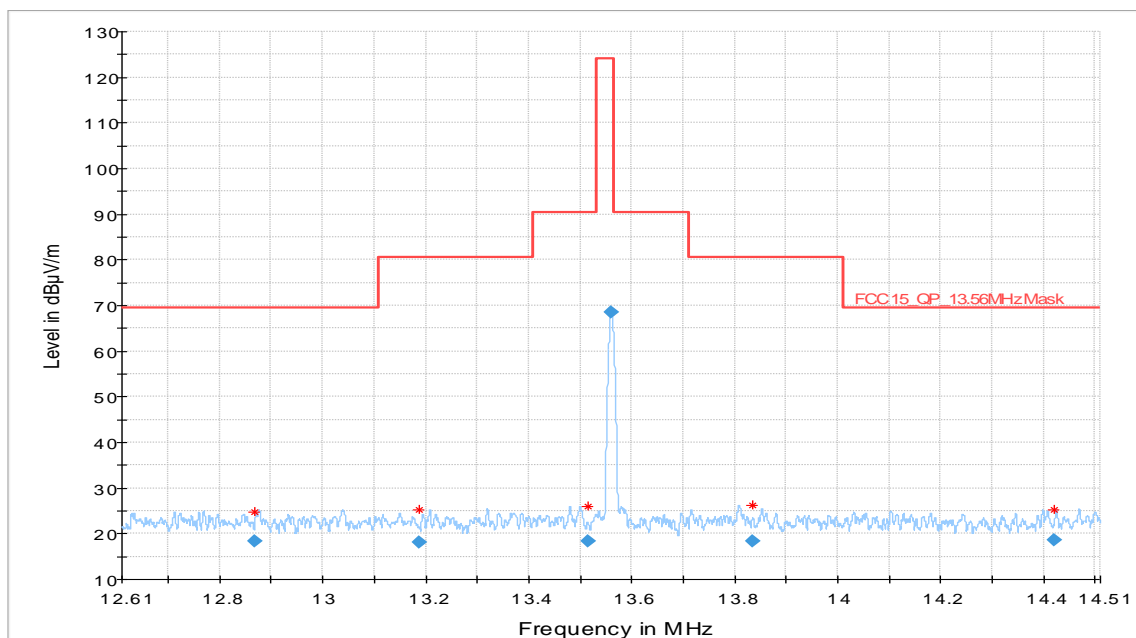
Figure 3: Out of Band Spectrum Mask for RFID Reader – 0 Degree Loop Antenna X-axis
