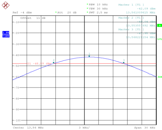
Figure 29: Frequency Stability at 40 °C - Start
