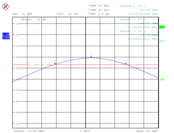
Figure 7: Frequency Stability at -20 °C – 5 min
