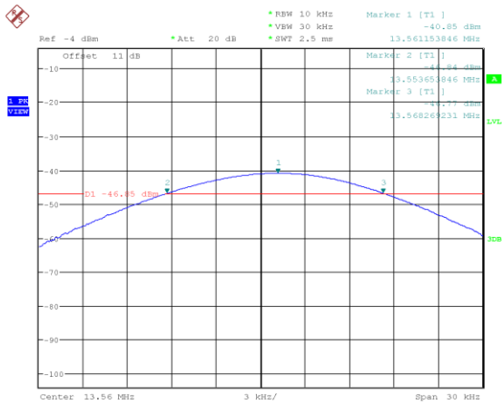
Figure 9: Frequency Stability at -10 °C - Start
