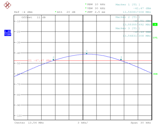
Figure 26: Frequency Stability at 30 °C – 2 min
