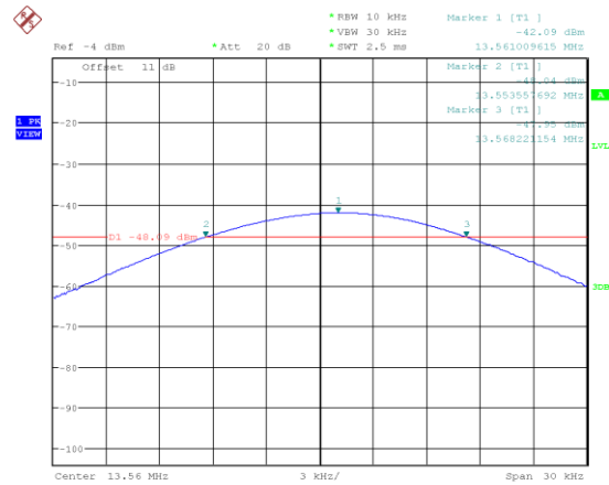
Figure 30: Frequency Stability at 40 °C – 2 min
