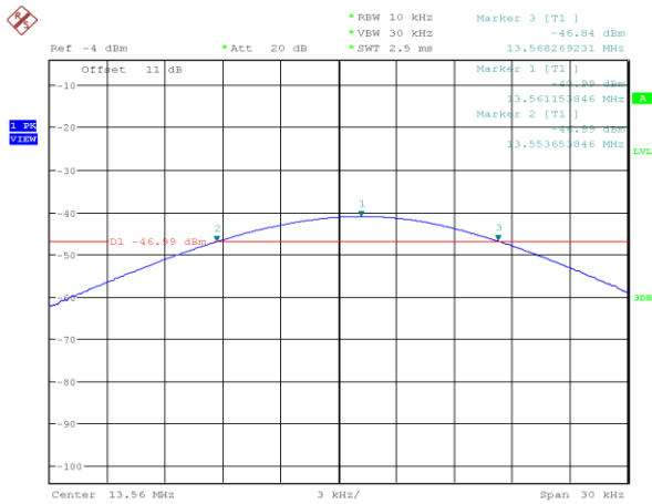
Figure 5: Frequency Stability at -20 °C - Start
