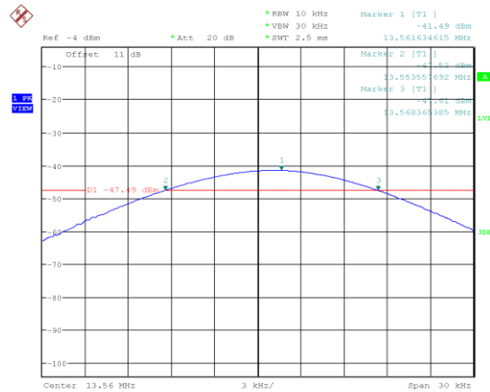
Figure 25: Frequency Stability at 30 °C - Start
