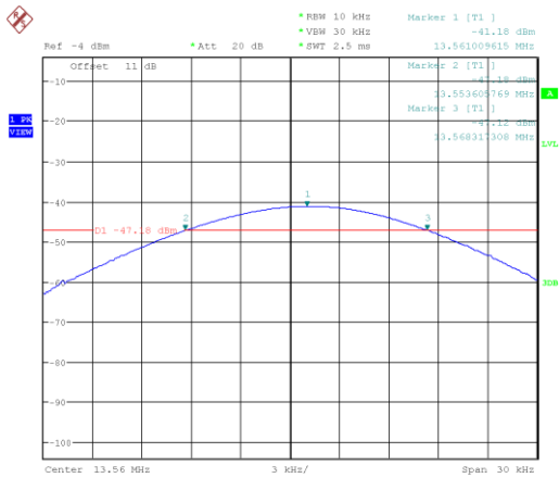
Figure 17: Frequency Stability at 10 °C - Start
