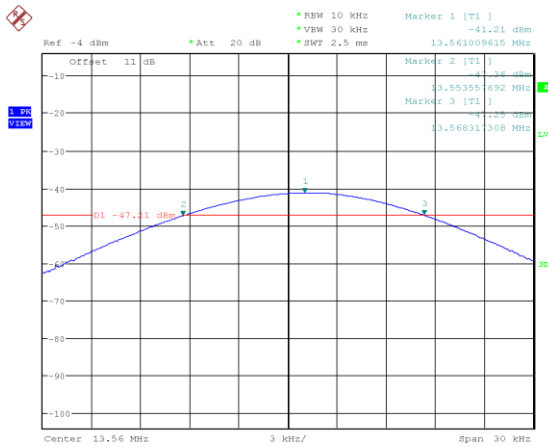
Figure 21: Frequency Stability at 20 °C - Start
