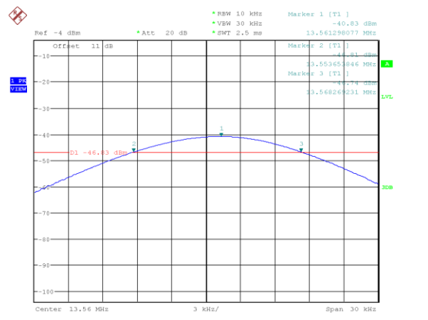
Figure 8: Frequency Stability at -20 °C – 10 min
