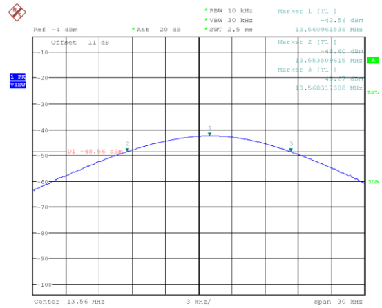
Figure 34: Frequency Stability at 50 °C - 2 min
