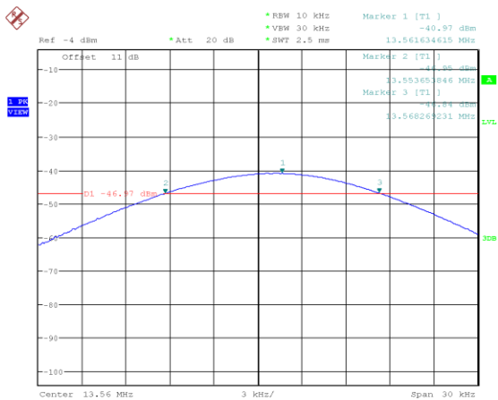
Figure 15: Frequency Stability at 0 °C - 5 min
