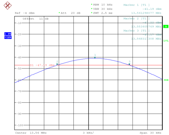
Figure 18: Frequency Stability at 10 °C – 2 min
