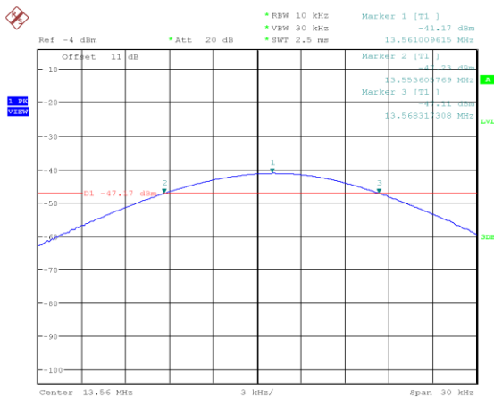
Figure 19: Frequency Stability at 10 °C – 5 min
