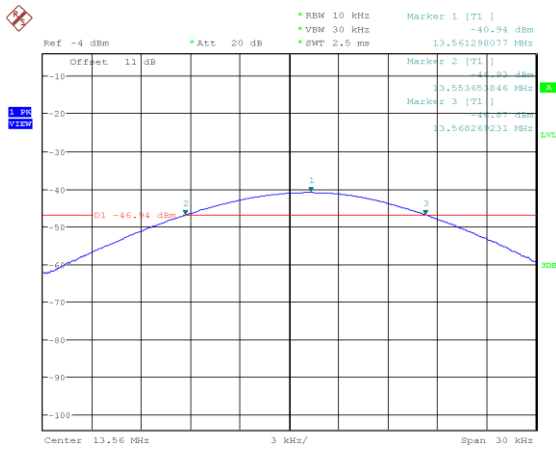
Figure 13: Frequency Stability at 0 °C - Start
