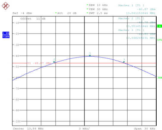
Figure 11: Frequency Stability at -10 °C – 5 min
