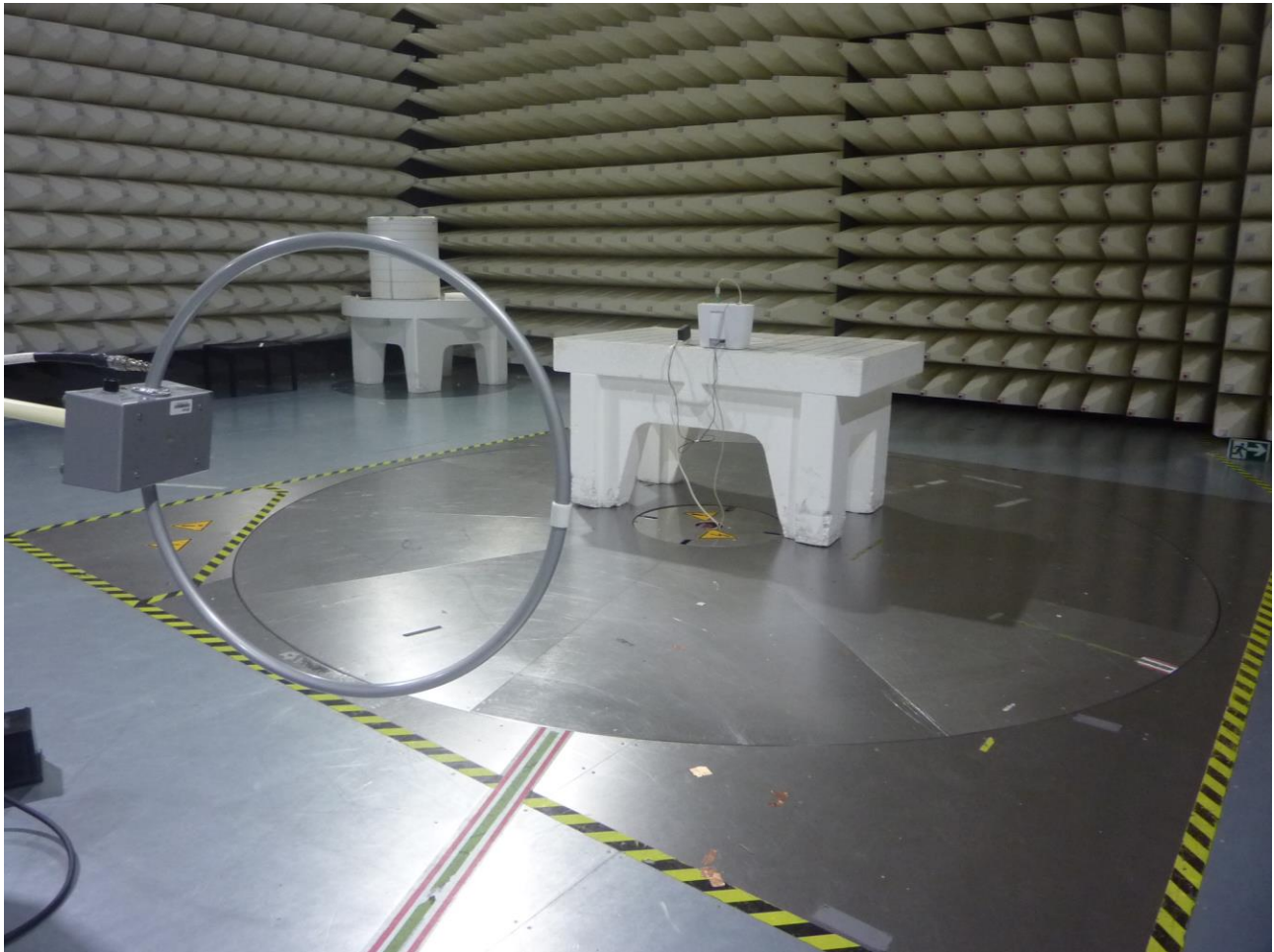
Figure 3: Test Setup for Radiated Emissions 9kHz to 30MHz (BT LE, RFID and Unintentional Modes)
