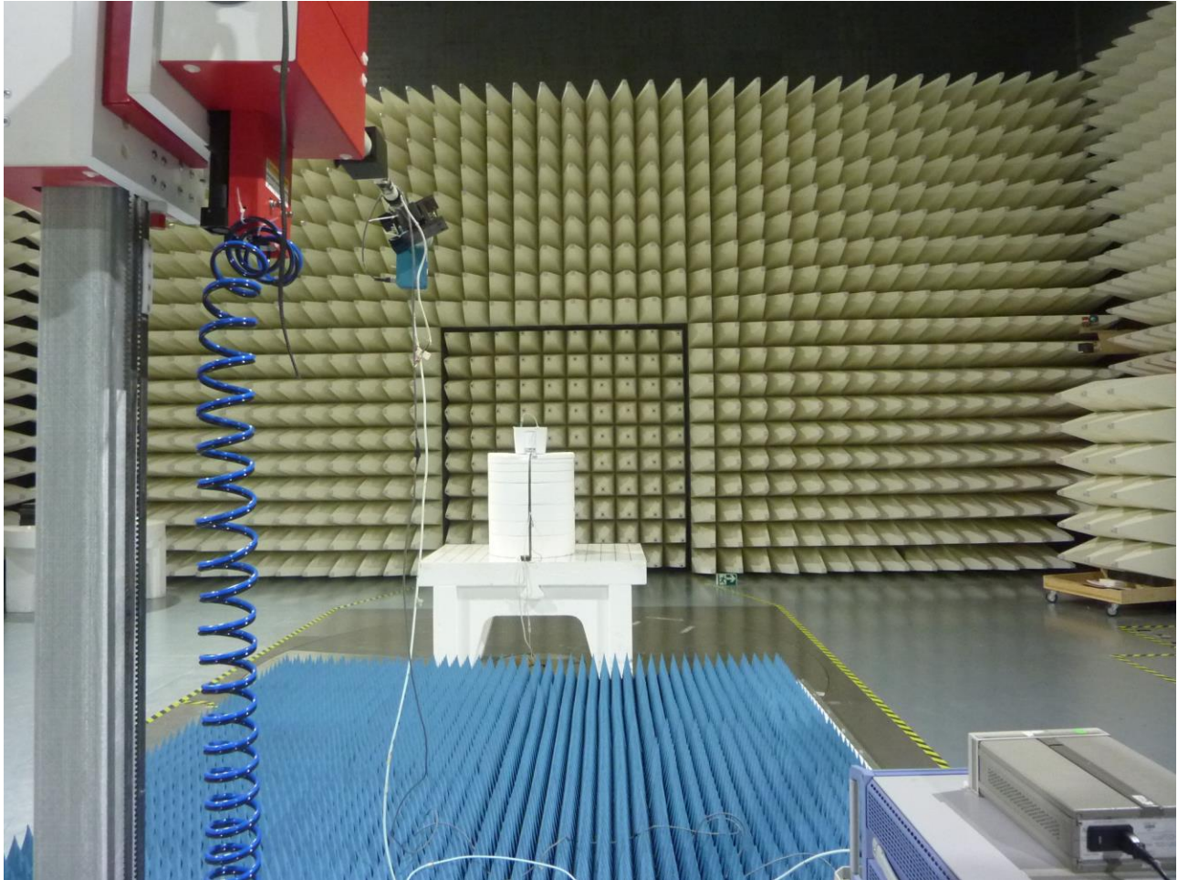
Figure 6: Test Setup for Radiated Emissions 18GHz to 26 GHz (BT LE Modes)
