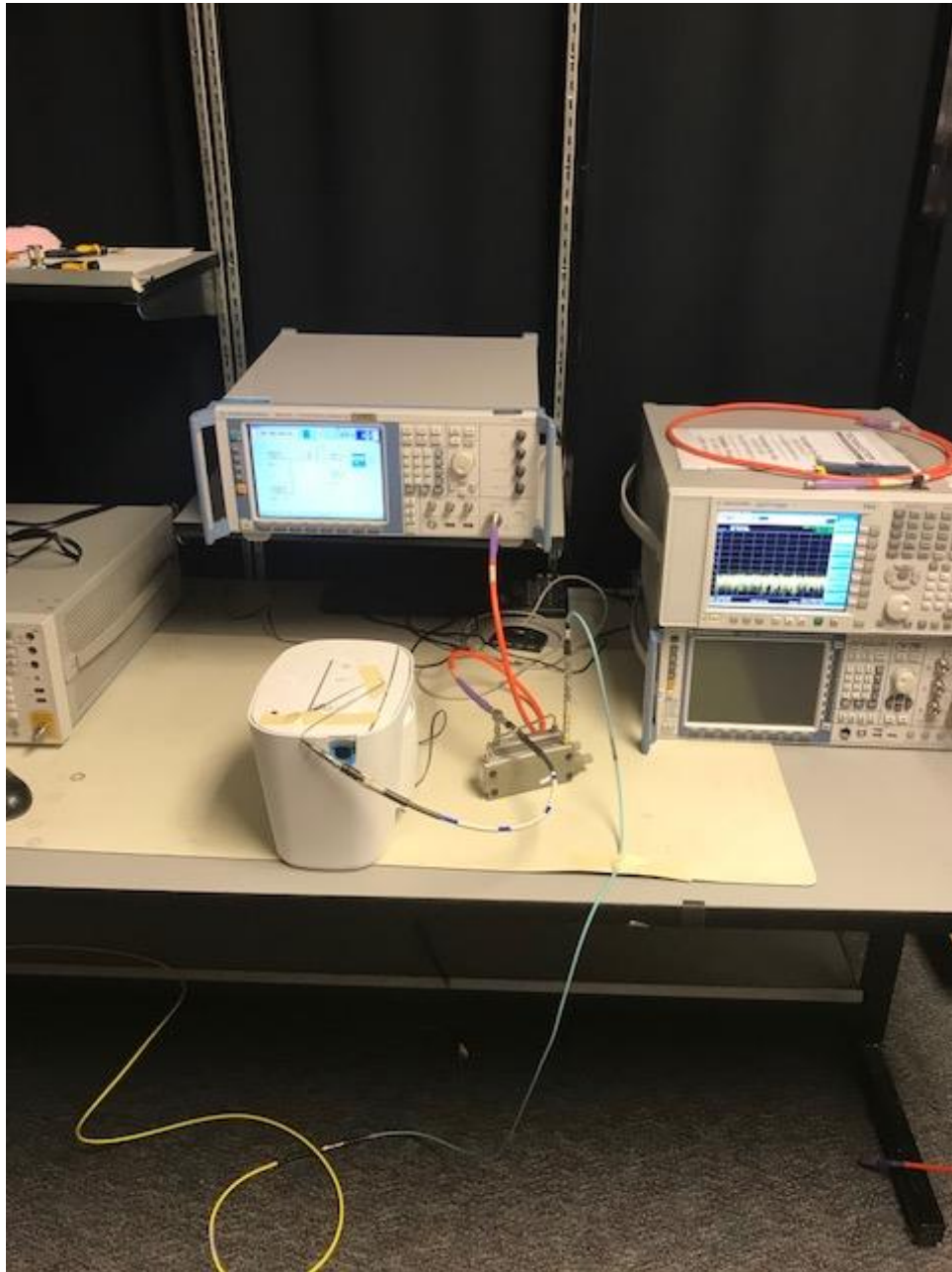
Figure 8: Test Setup for Conducted (BT LE Modes)
