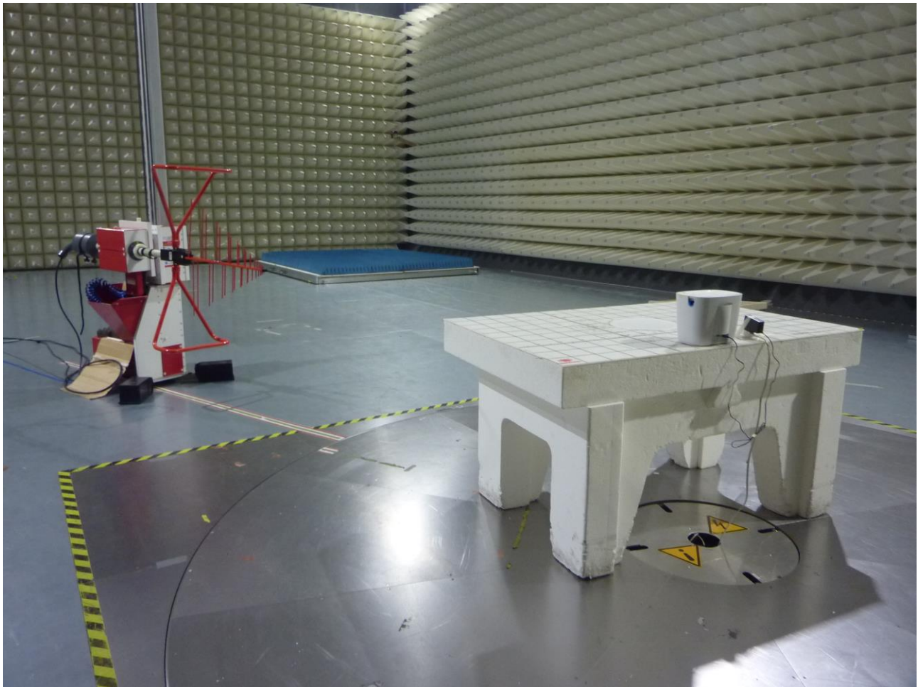
Figure 4: Test Setup for Radiated Emissions 30MHz to 1000MHz (BT LE, RFID and Unintentional Modes)
