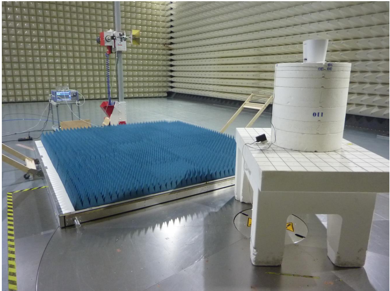
Figure 5: Test Setup for Radiated Emissions 1GHz to 18GHz (BT LE and RFID)
