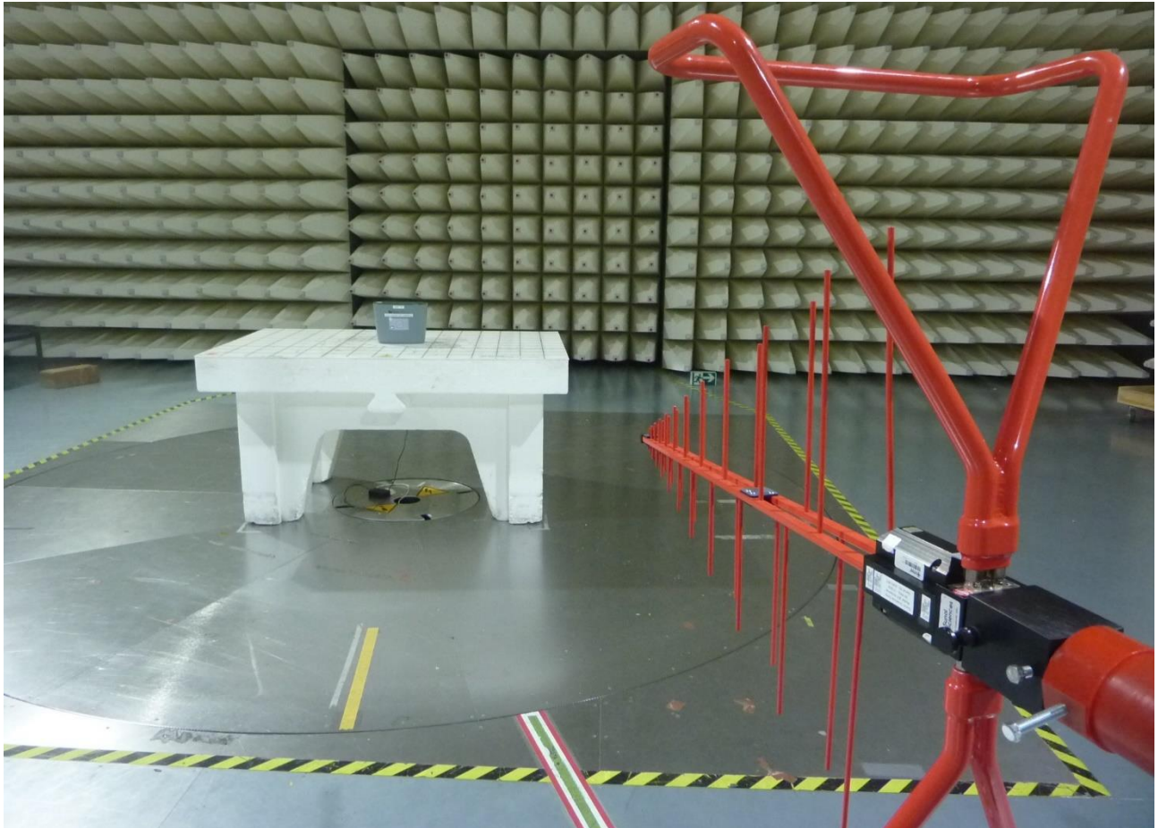
Figure 6: Test Setup for Radiated Emissions 30MHz to 1000MHz (BLE) - Front View
