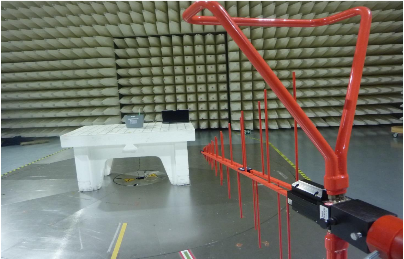
Figure 4: Test Setup for Radiated Emissions 30MHz to 1000MHz (RFID) - Front View
