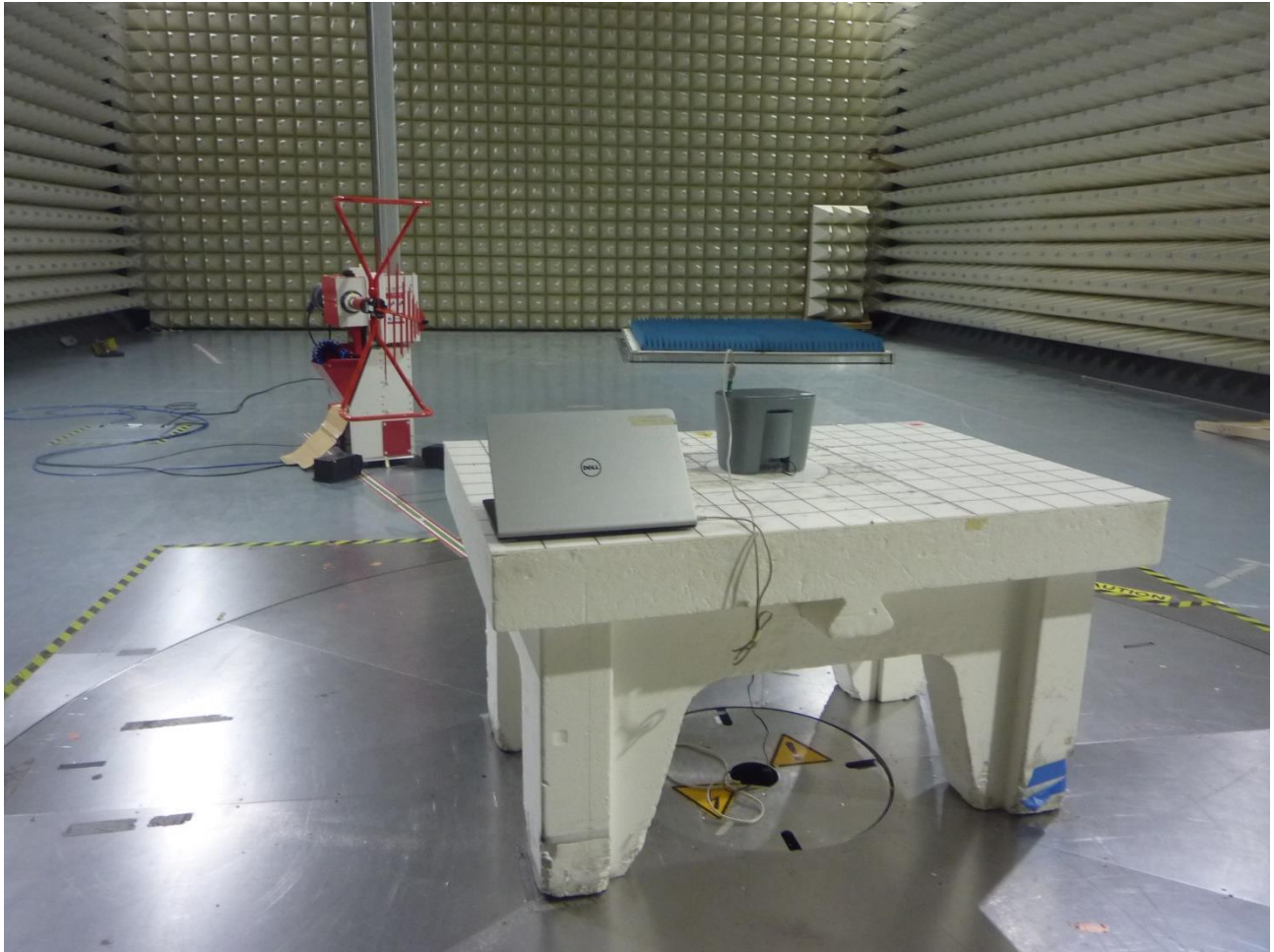
Figure 5: Test Setup for Radiated Emissions 30MHz to 1000MHz (RFID) - Rear View
