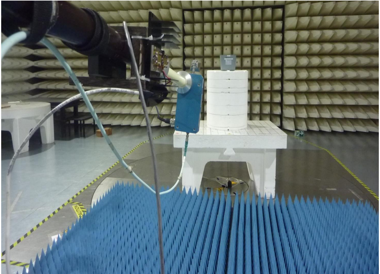
Figure 10: Test Setup for Radiated Emissions 18GHz to 26 GHz (BLE Modes)- Front View
