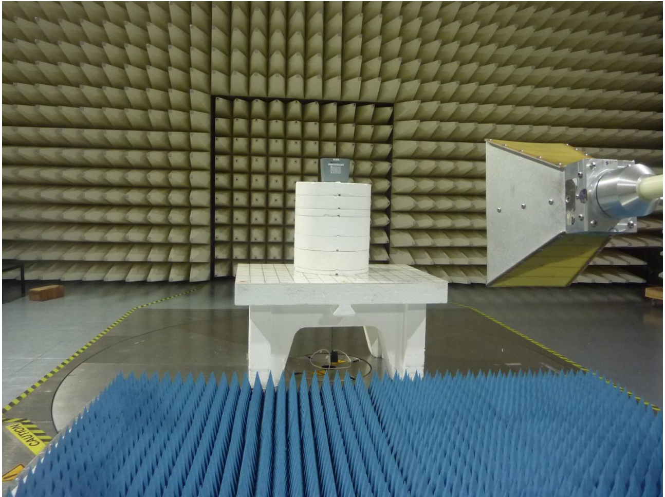
Figure 8: Test Setup for Radiated Emissions 1GHz to 18GHz (BLE) - Front View
