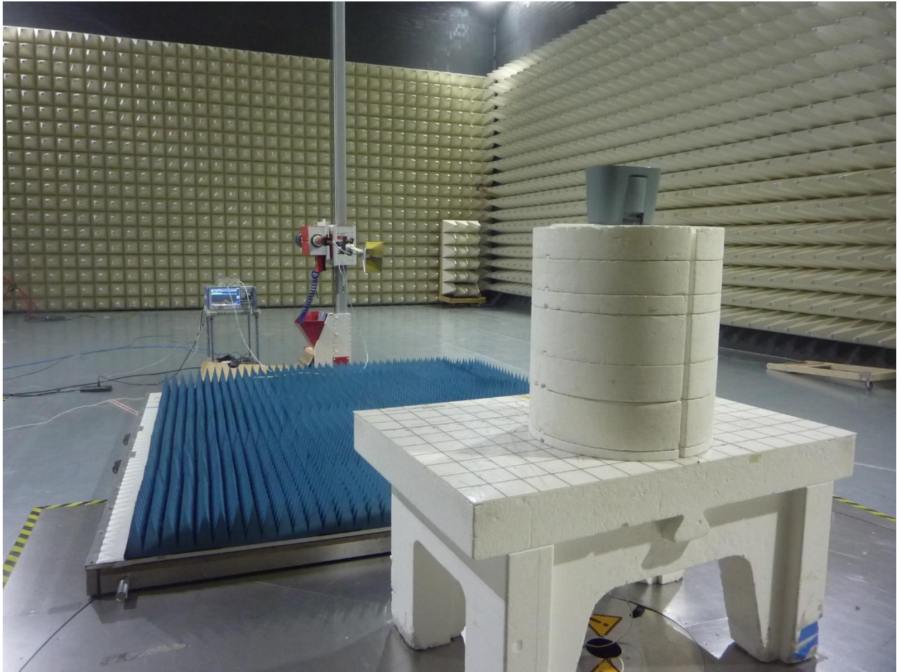
Figure 9: Test Setup for Radiated Emissions 1GHz to 18GHz (BLE)-Rear View
