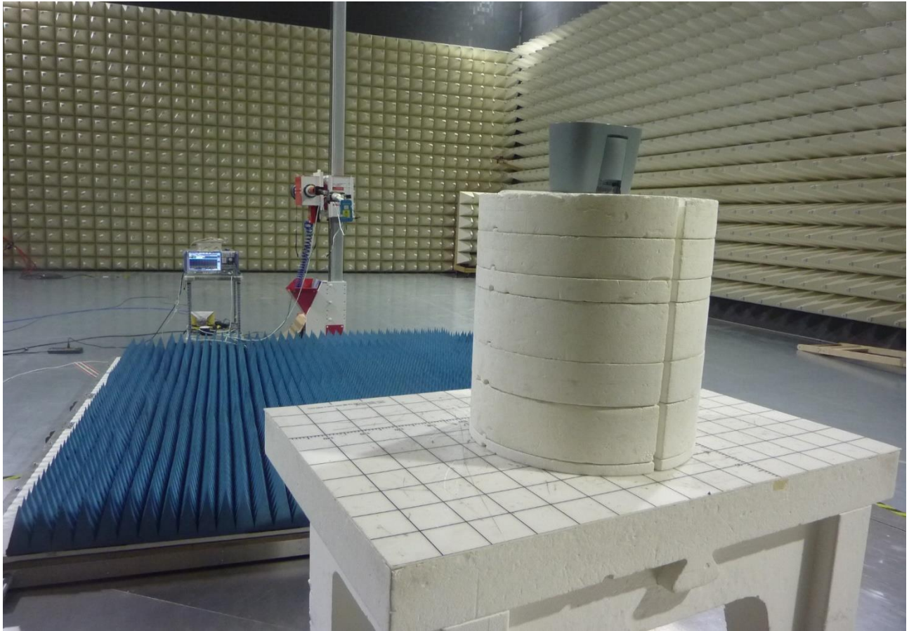
Figure 11: Test Setup for Radiated Emissions 18GHz to 26 GHz (BLE Modes)- Rear View
