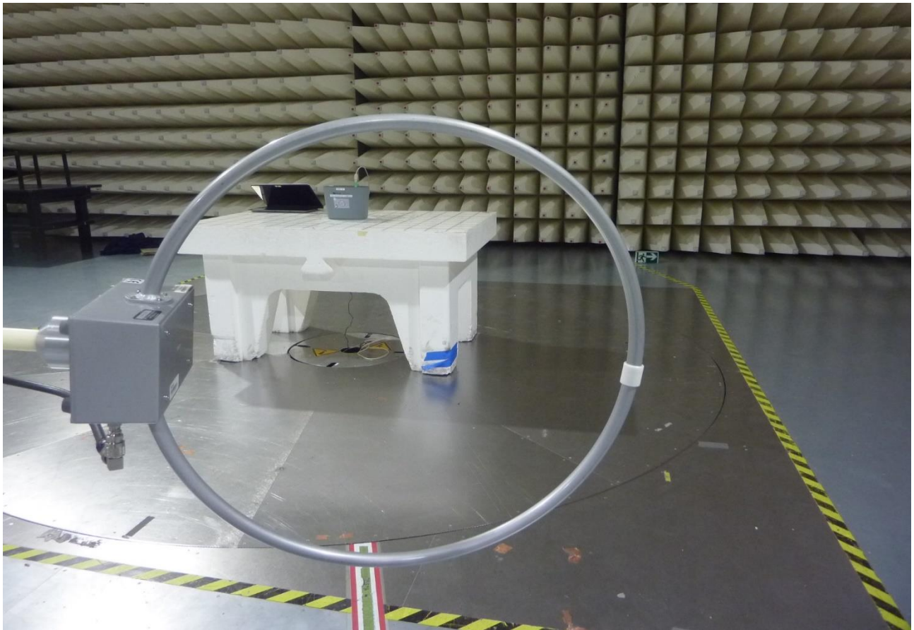
Figure 3: Test Setup for Radiated Emissions 9kHz to 30MHz (BLE and RFID)
