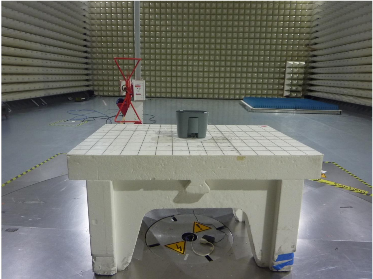
Figure 7: Test Setup for Radiated Emissions 30MHz to 1000MHz (BLE) - Rear View
