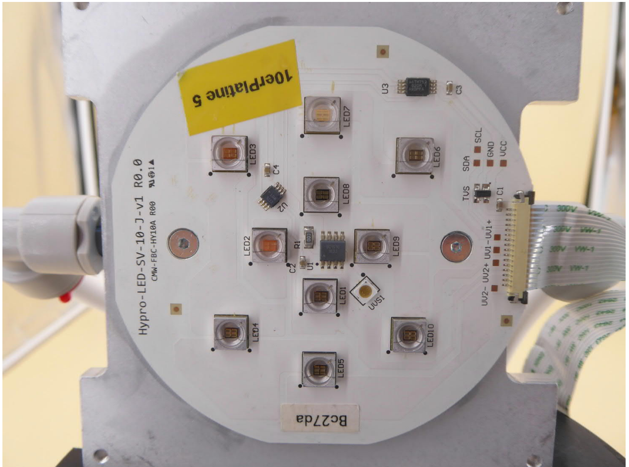
UV LED PCB (for disinfection)
