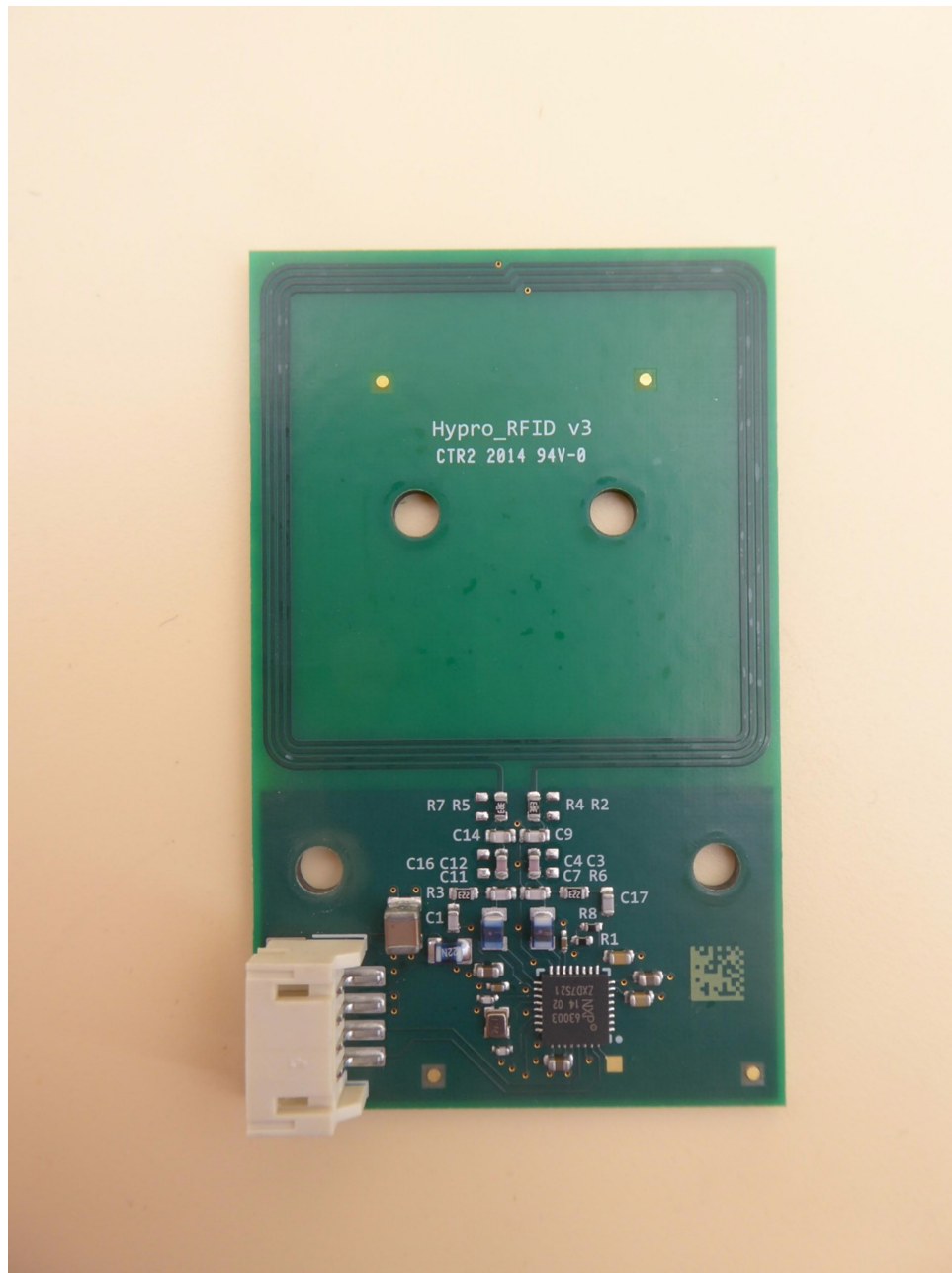
RFID PCB, top view
