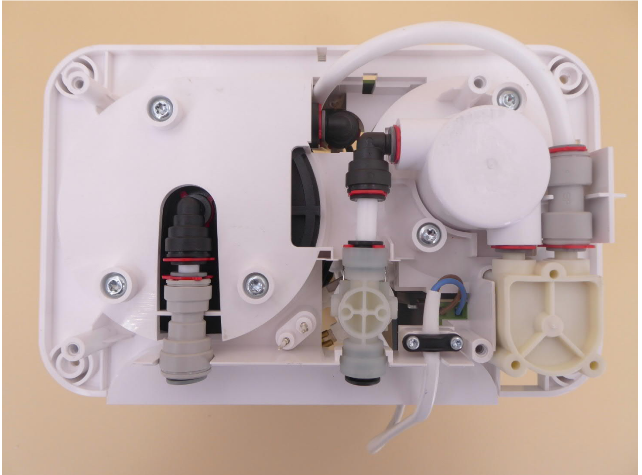
EUT, bottom view, bottom cover removed
