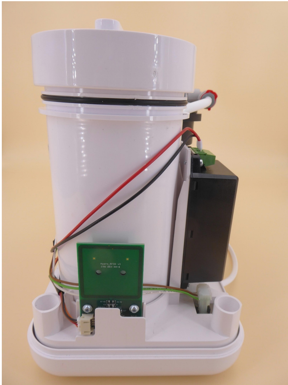
EUT, right side (RFID PCB)
