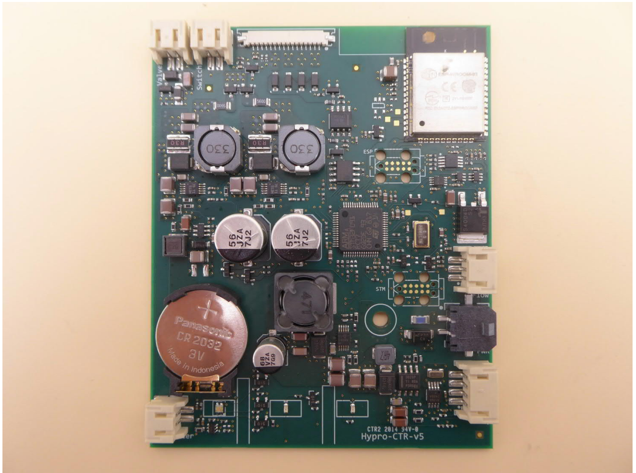
Main PCB, top view
