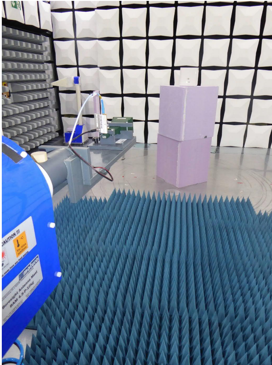
Test setup – radiated test in anechoic chamber (M276)
