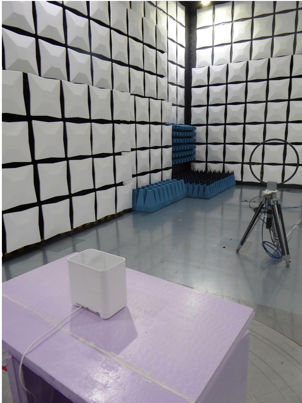
Test setup semi-anechoic chamber M276, 9 kHz - 30 MHz
