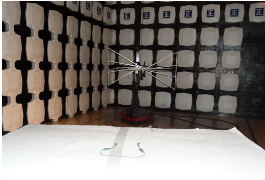
Measurement of Radiated Emission Test Set Up
