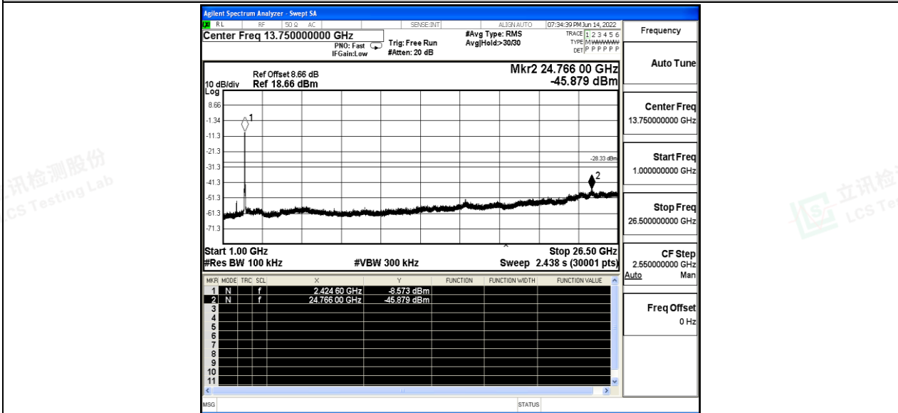
11N40SISO_Ant_2437_0~Reference
