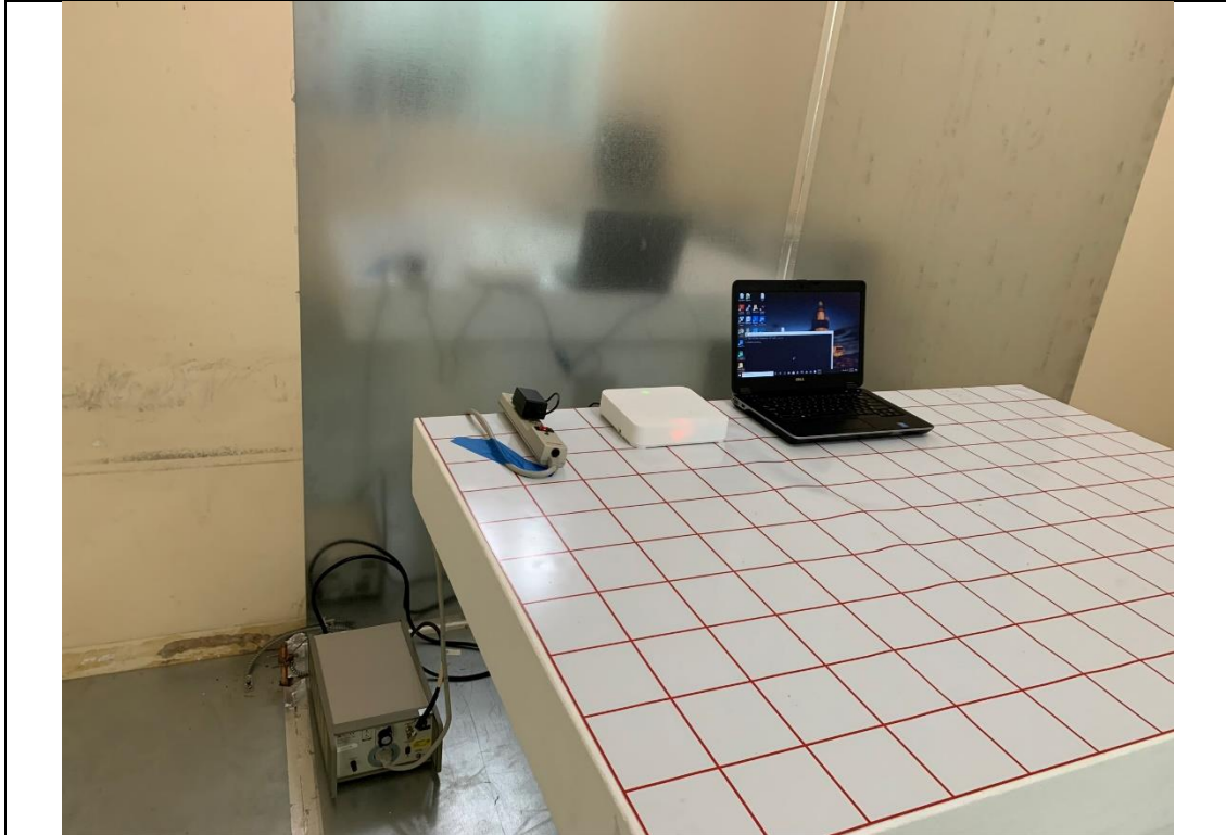
Conducted Emission setup – Front
