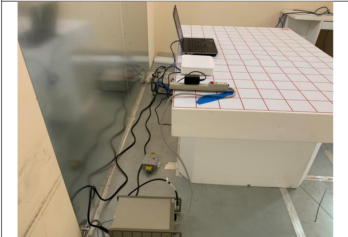
Conducted Emission setup – Rear
