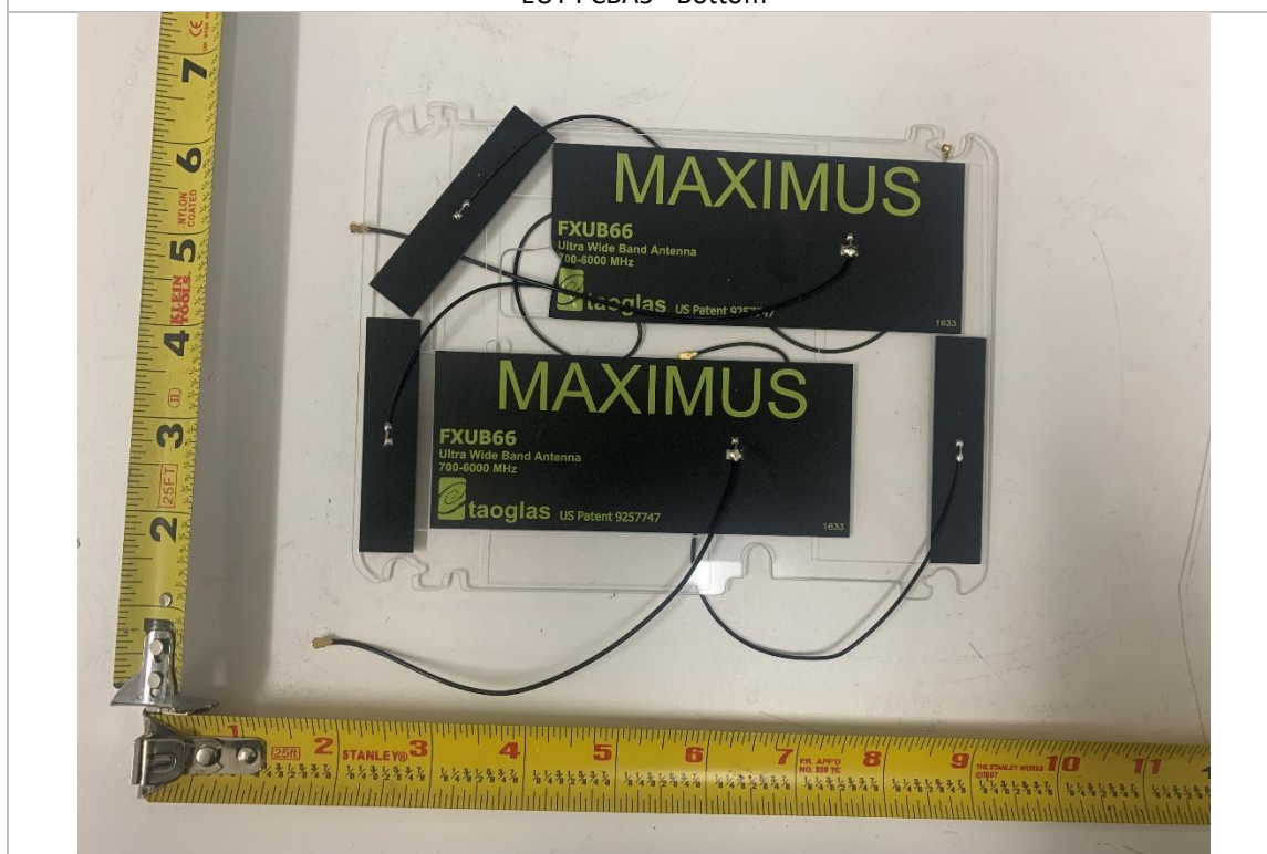
EUT Antenna (TX and RX) - Top
