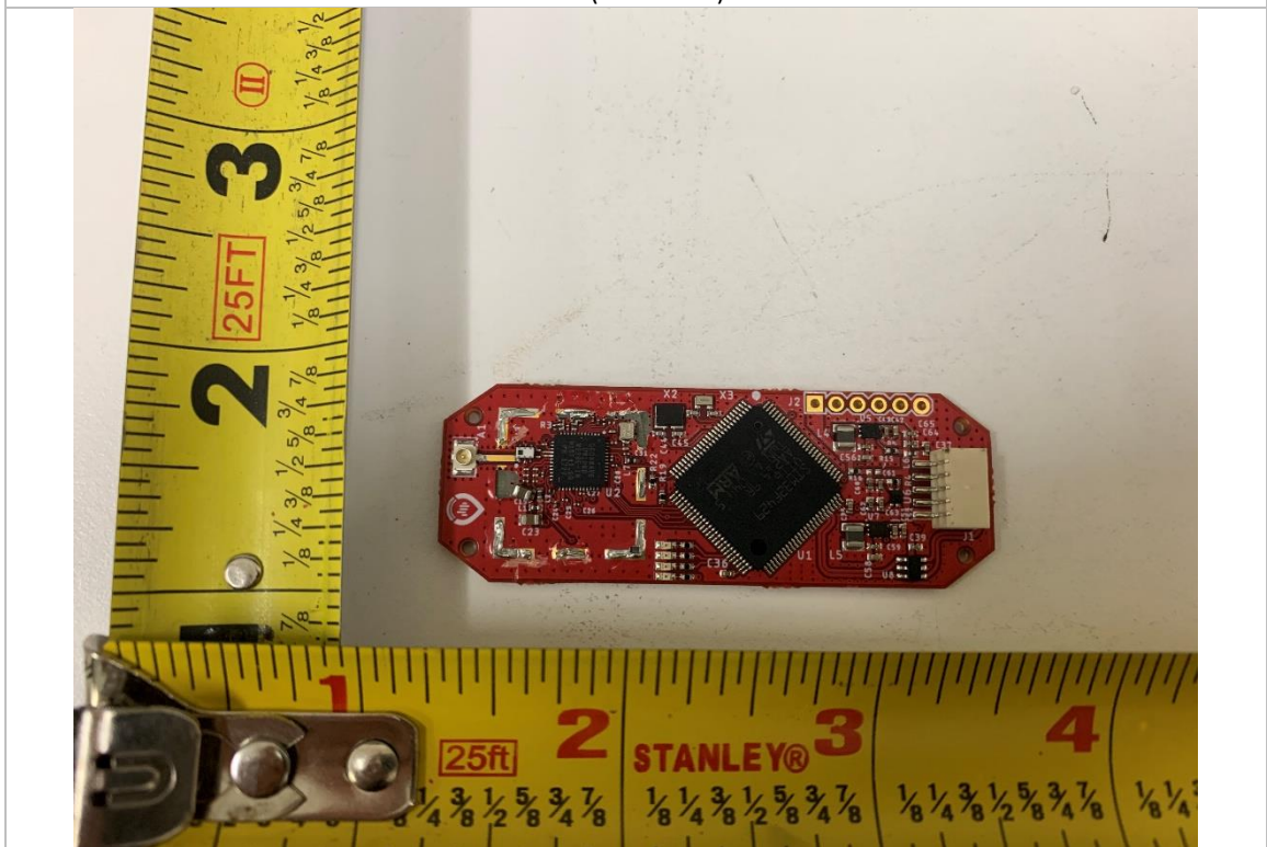
UWB Module – Top (without shielding)
