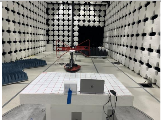
Radiated Emission Test below 1GHz Rear View
