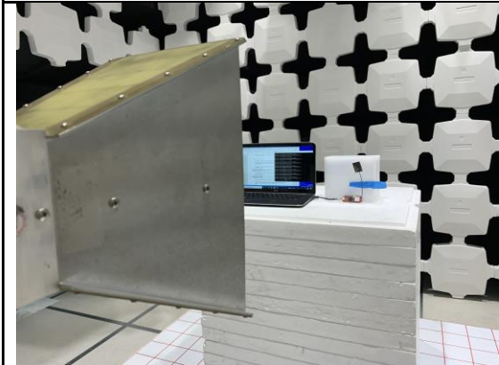
Radiated Emission Test above 1GHz Front View
