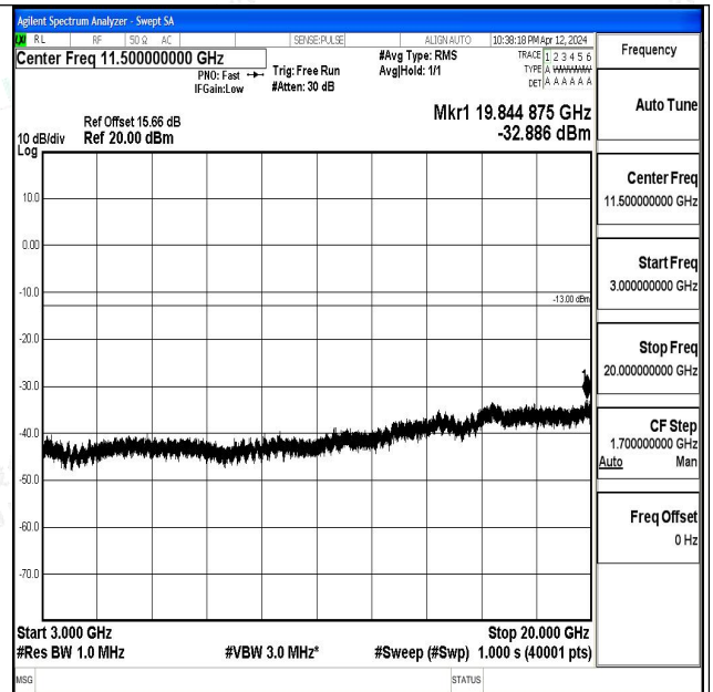
Band66_5MHz_16QAM_132647_1RB#0_3000~20000_3 000~20000
