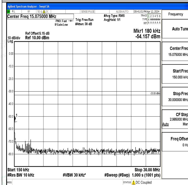
Band66_1.4MHz_16QAM_131979_1RB#0_0.15~30_0.15~30
