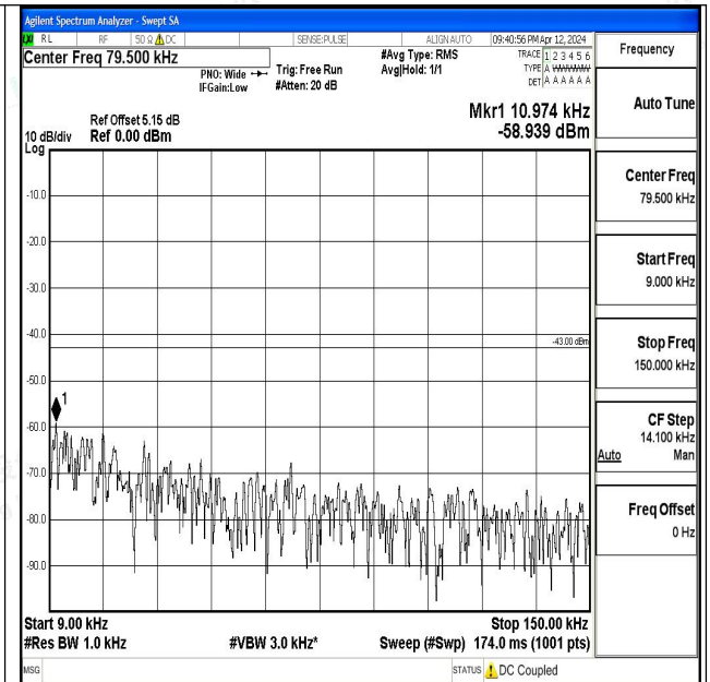
Band66_1.4MHz_16QAM_131979_1RB#0_0.009~0.15_0.009~0.15
