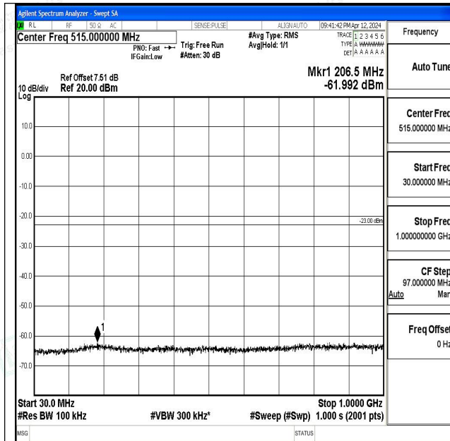
Band66_1.4MHz_QPSK_132322_1RB#0_30~1000_30~1 000
