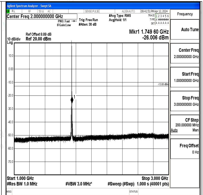
Band66_1.4MHz_QPSK_132322_1RB#0_1000~3000_10 00~3000
