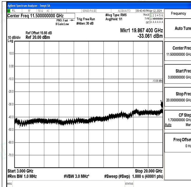
Band66_1.4MHz_QPSK_131979_1RB#0_3000~20000_3 000~20000
