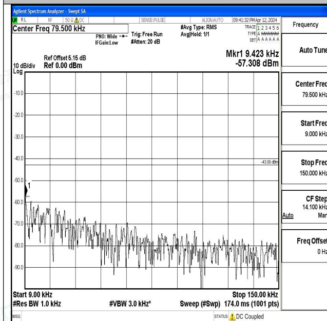
Band66_1.4MHz_QPSK_132322_1RB#0_0.009~0.15_0.009~0.15
