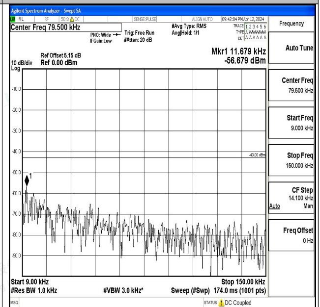
Band66_1.4MHz_16QAM_132322_1RB#0_0.009~0.15_ 0.009~0.15
