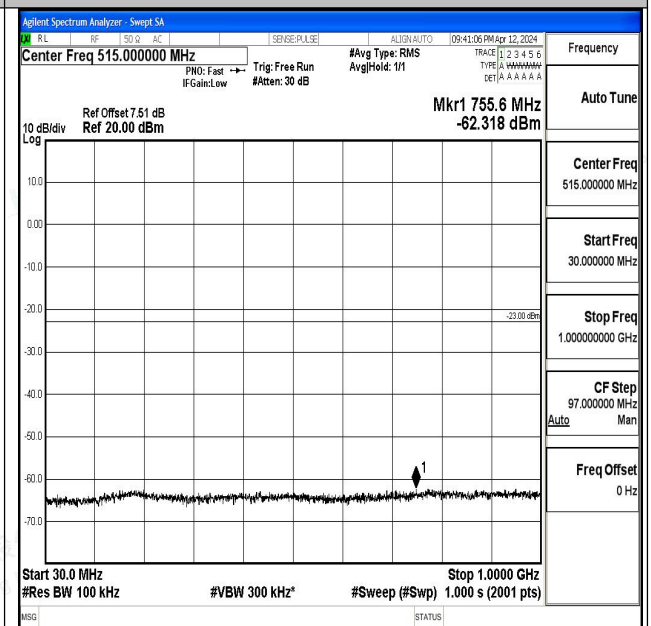
Band66_1.4MHz_16QAM_131979_1RB#0_30~1000_30~1000
