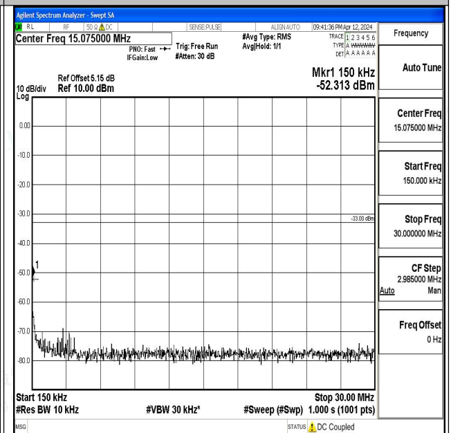
Band66_1.4MHz_QPSK_132322_1RB#0_0.15~30_0.15~30
