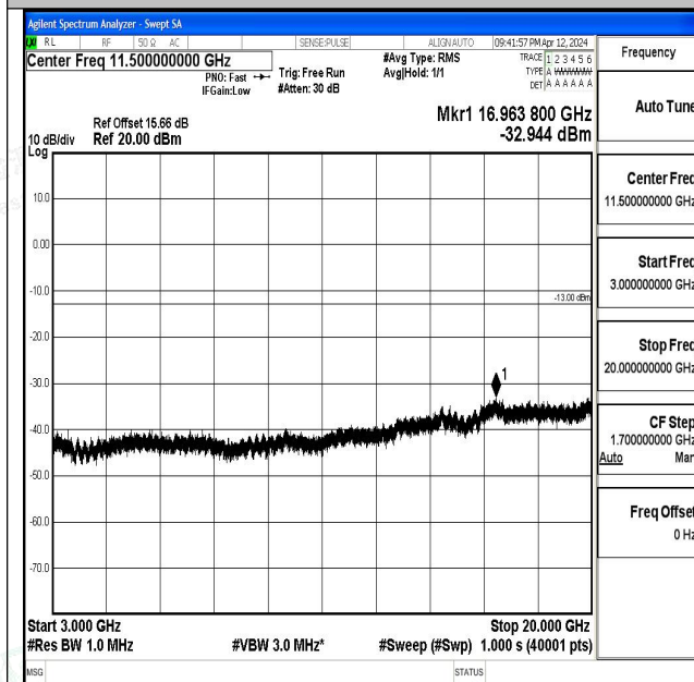
Band66_1.4MHz_QPSK_132322_1RB#0_3000~20000_3 000~20000
