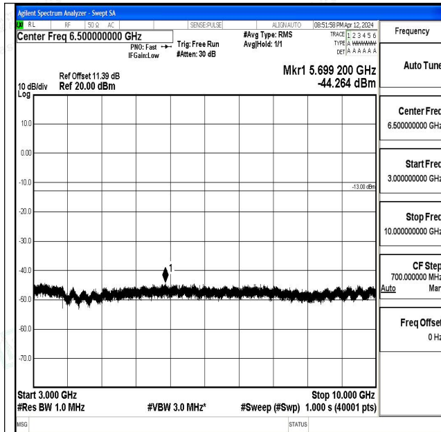
Band17_5MHz_QPSK_23755_1RB#0_3000~10000_300 0~10000
