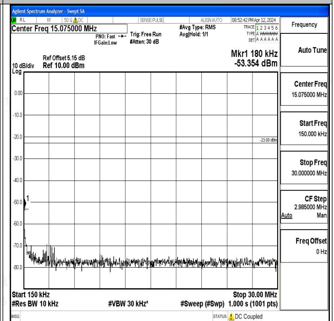
Band17_5MHz_QPSK_23790_1RB#0_0.15~30_0.15~30
