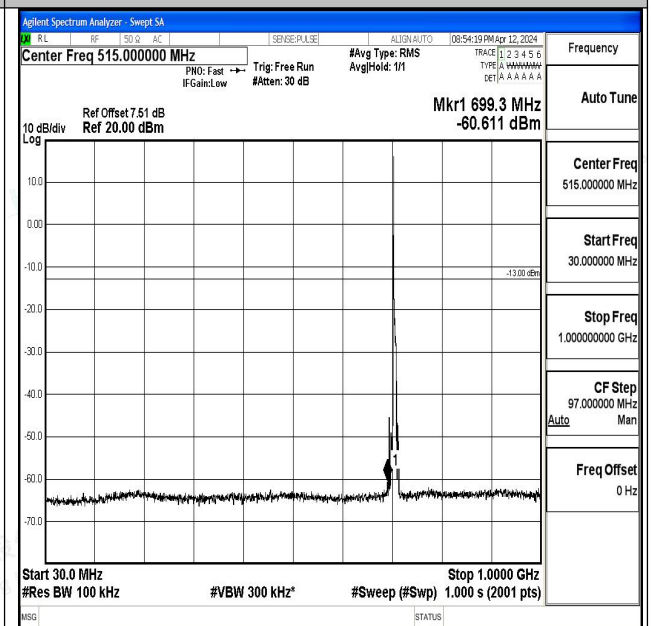
Band17_5MHz_16QAM_23825_1RB#0_30~1000_30~10 00
