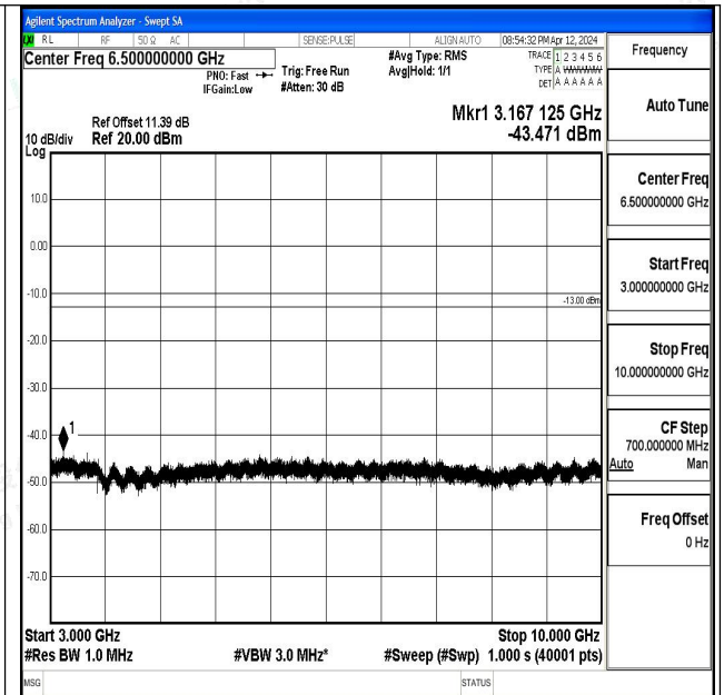
Band17_5MHz_16QAM_23825_1RB#0_3000~10000_30 00~10000
