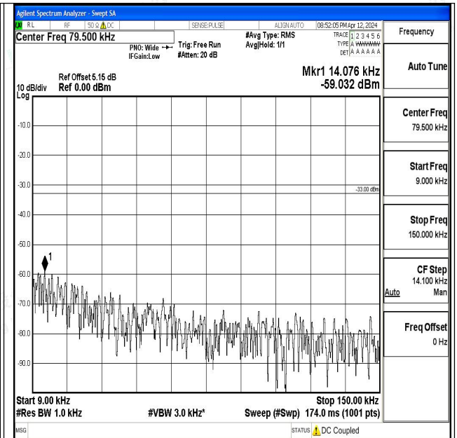
Band17_5MHz_16QAM_23755_1RB#0_0.009~0.15_0.0 09~0.15
