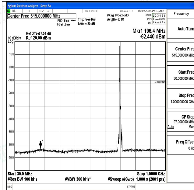
Band17_10MHz_QPSK_23780_1RB#0_30~1000_30~10 00
