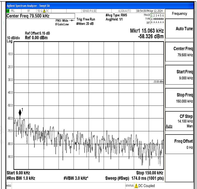
Band17_5MHz_16QAM_23825_1RB#0_0.009~0.15_0.0 09~0.15
