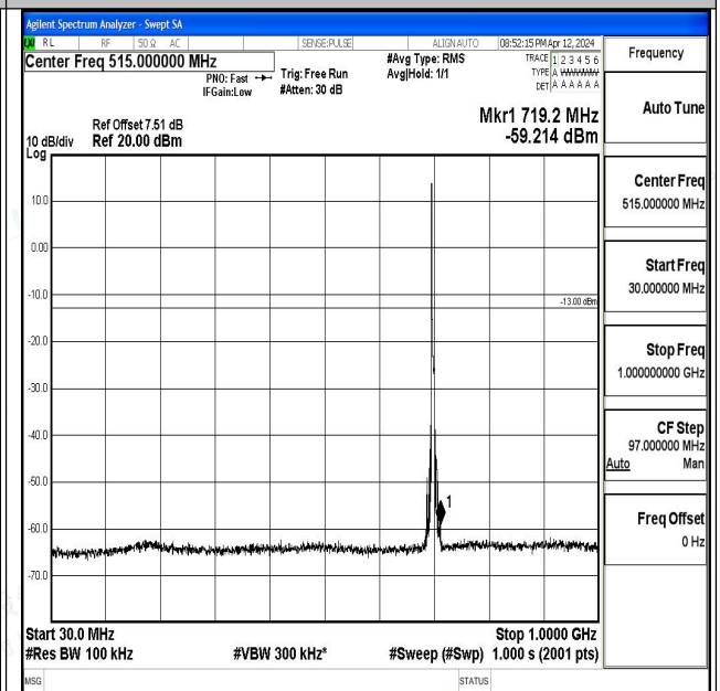
Band17_5MHz_16QAM_23755_1RB#0_30~1000_30~10 00
