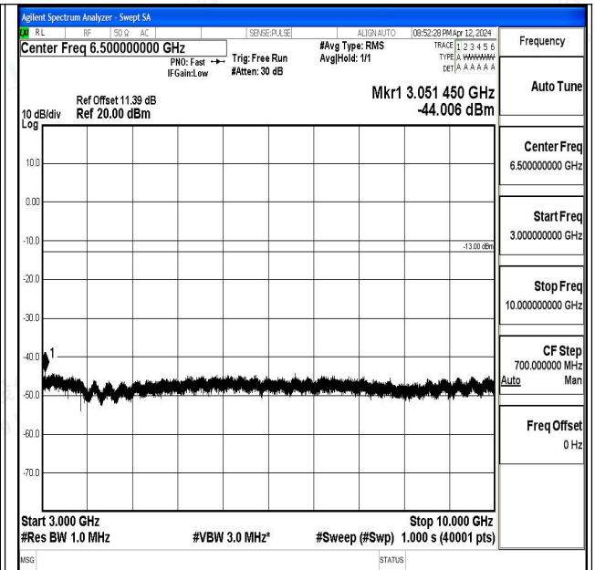
Band17_5MHz_16QAM_23755_1RB#0_3000~10000_30 00~10000
