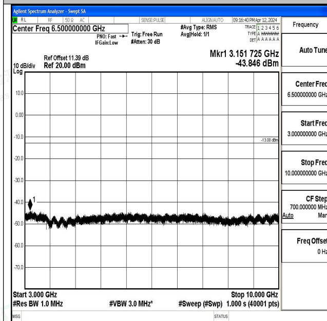
Band17_10MHz_QPSK_23780_1RB#0_3000~10000_30 00~10000
