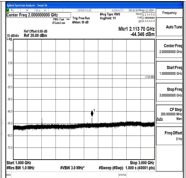
Band17_10MHz_QPSK_23780_1RB#0_1000~3000_100 0~3000
