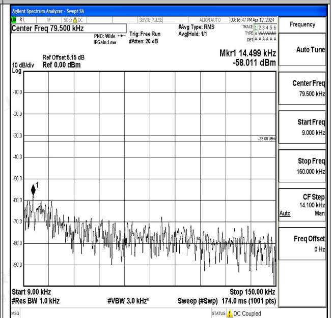
Band17_10MHz_16QAM_23780_1RB#0_0.009~0.15_0. 009~0.15
