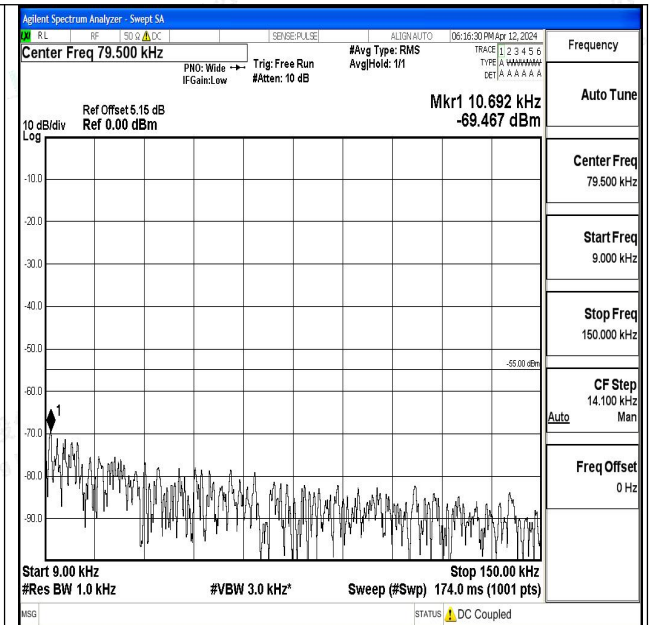
Band7_15MHz_16QAM_20825_1RB#0_0.009~0.15_0.0 09~0.15
