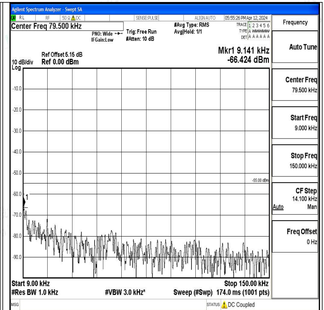
Band7_10MHz_16QAM_21100_1RB#0_0.009~0.15_0.00 9~0.15
