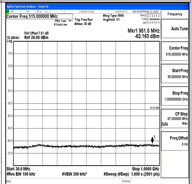
Band7_15MHz_16QAM_20825_1RB#0_30~1000_30~10 00
