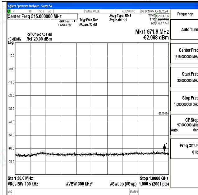
Band7_15MHz_QPSK_21100_1RB#0_30~1000_30~100
