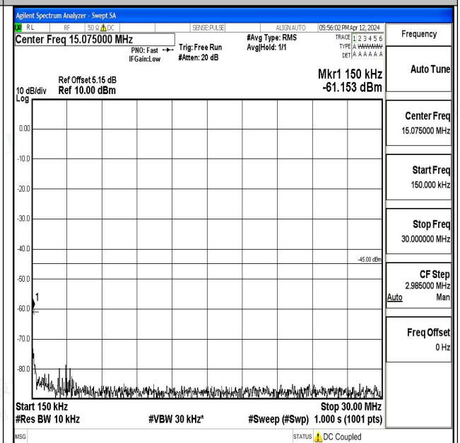
Band7_10MHz_QPSK_21400_1RB#0_0.15~30_0.15~30
