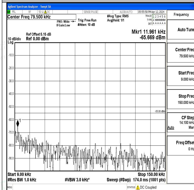
Band7_10MHz_QPSK_21400_1RB#0_0.009~0.15_0.009 ~0.15
