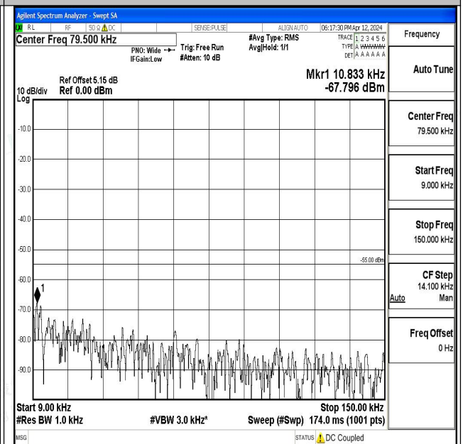
Band7_15MHz_16QAM_21100_1RB#0_0.009~0.15_0.00
