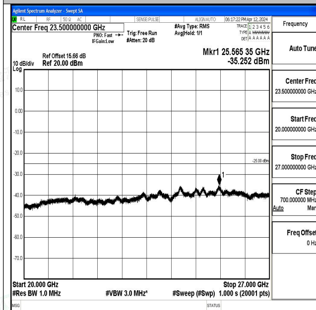
Band7_15MHz_QPSK_21100_1RB#0_20000~27000_20
