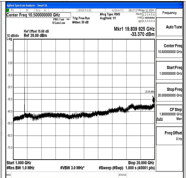
Band7_15MHz_QPSK_21100_1RB#0_1000~20000_100
