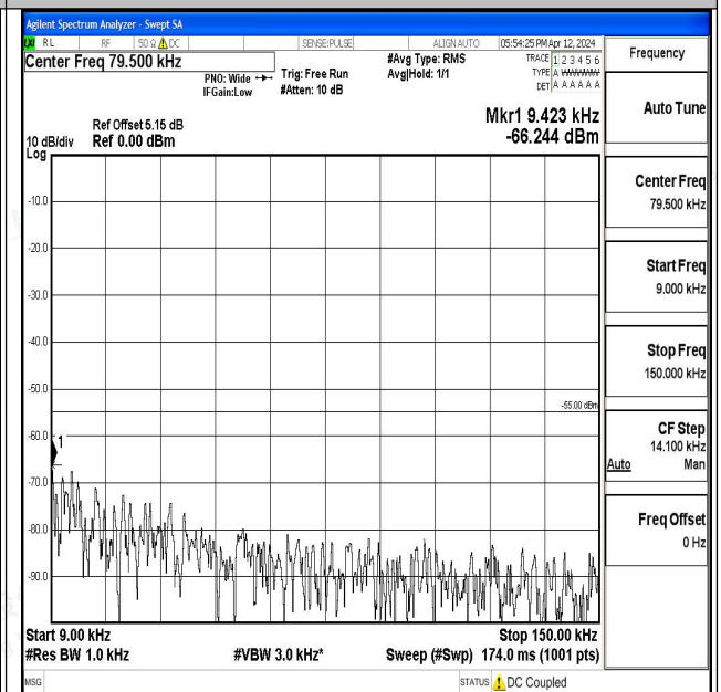
Band7_10MHz_16QAM_20800_1RB#0_0.009~0.15_0.0 09~0.15
