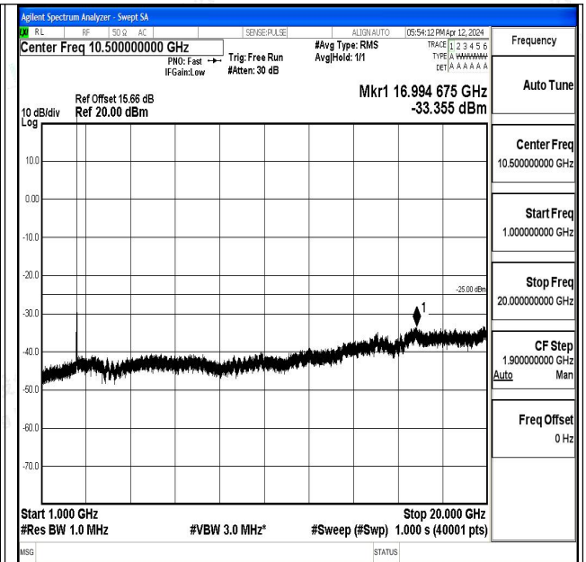
Band7_10MHz_QPSK_20800_1RB#0_1000~20000_100 0~20000
