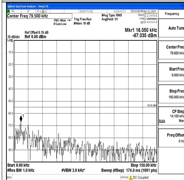
Band7_10MHz_QPSK_20800_1RB#0_0.009~0.15_0.009 ~0.15
