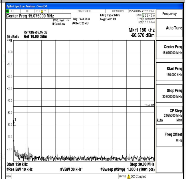
Band7_10MHz_QPSK_20800_1RB#0_0.15~30_0.15~30
