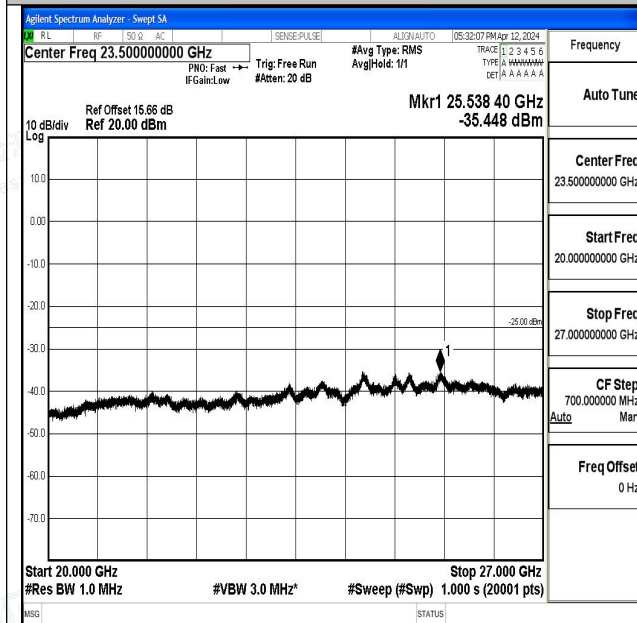
Band7_5MHz_QPSK_21100_1RB#0_20000~27000_20000~27000
