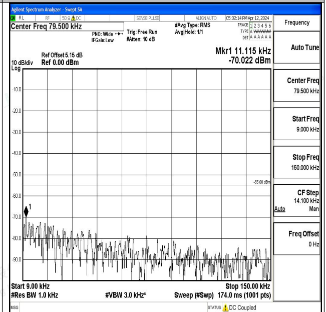
Band7_5MHz_16QAM_21100_1RB#0_0.009~0.15_0.009~0.15
