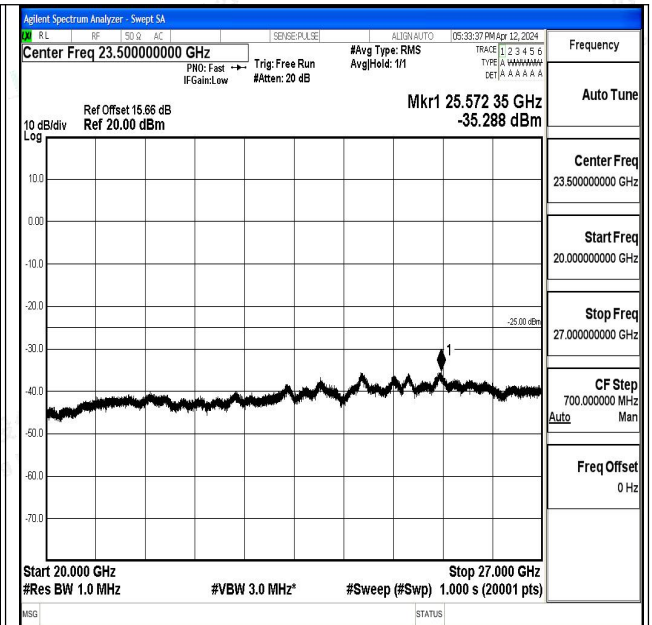
Band7_5MHz_16QAM_21425_1RB#0_20000~27000_20 000~27000
