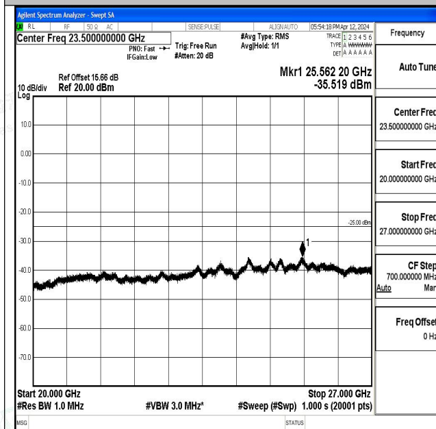
Band7_10MHz_QPSK_20800_1RB#0_20000~27000_20 000~27000
