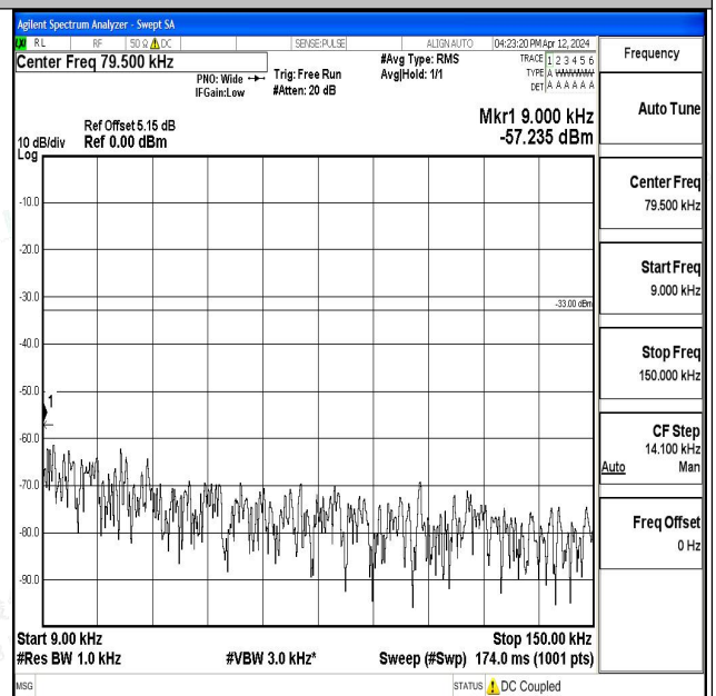
Band5_3MHz_16QAM_20635_1RB#0_0.009~0.15_0.009~0.15
