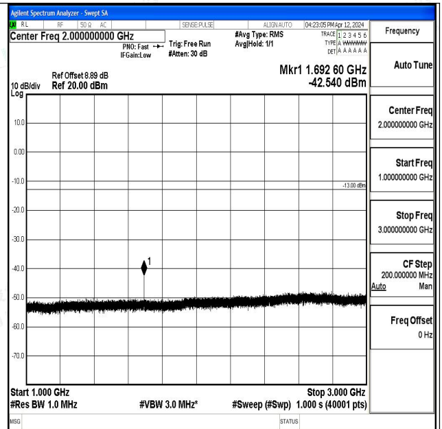
Band5_3MHz_QPSK_20635_1RB#0_1000~3000_1000~3000
