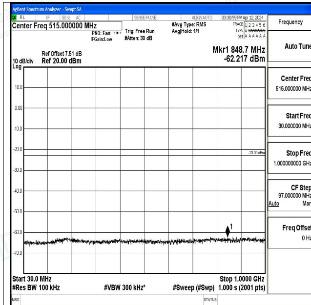
Band4_20MHz_QPSK_20050_1RB#0_30~1000_30~100 0
