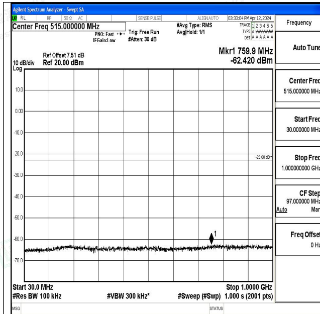
Band4_20MHz_QPSK_20300_1RB#0_30~1000_30~100 0
