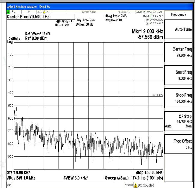
Band4_20MHz_16QAM_20300_1RB#0_0.009~0.15_0.0 09~0.15
