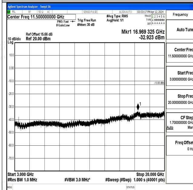
Band4_20MHz_QPSK_20300_1RB#0_3000~20000_300 0~20000
