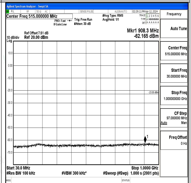
Band4_5MHz_16QAM_20375_1RB#0_30~1000_30~1000 0
