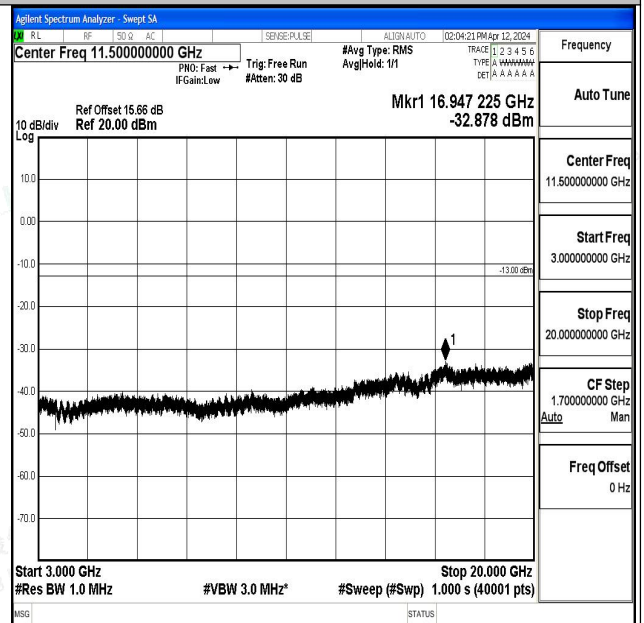
Band4_3MHz_16QAM_19965_1RB#0_3000~20000_3000 0~20000
