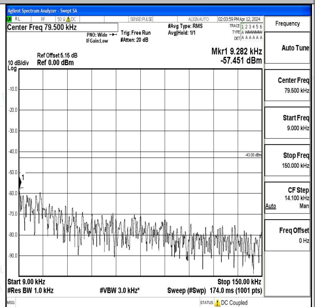
Band4_3MHz_16QAM_19965_1RB#0_0.009~0.15_0.009~0.15
