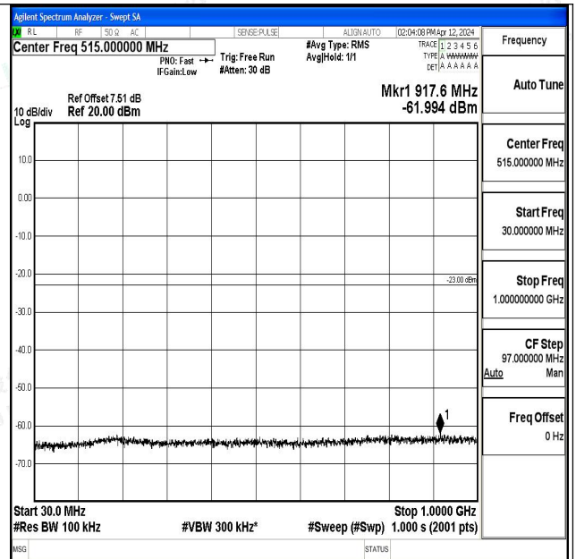
Band4_3MHz_16QAM_19965_1RB#0_30~1000_30~1000 0
