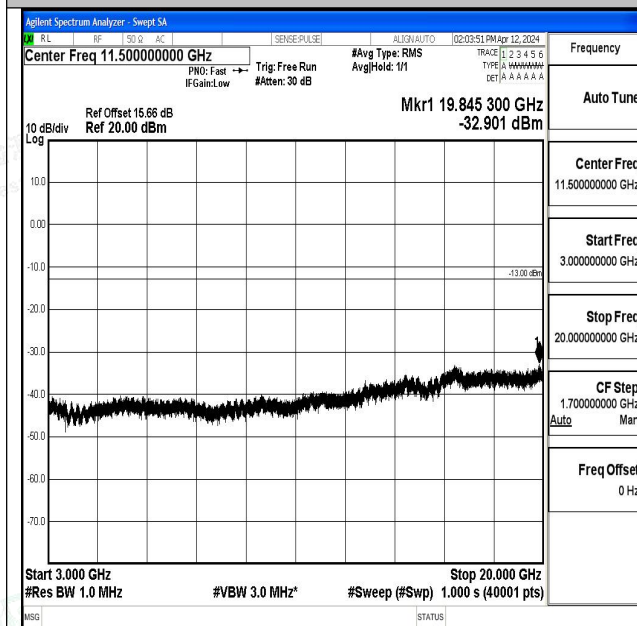
Band4_3MHz_QPSK_19965_1RB#0_3000~20000_3000~20000
