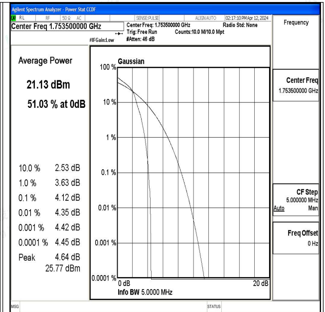
Band4-3MHz-16QAM-20385-1RB#0-PASS
