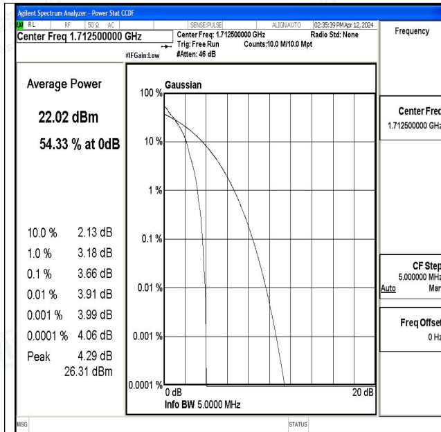
Band4-5MHz-QPSK-19975-1RB#0-PASS
