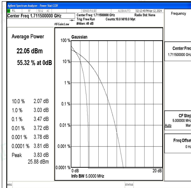
Band4-3MHz-QPSK-19965-1RB#0-PASS
