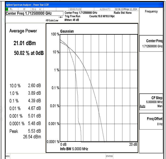
Band4-5MHz-16QAM-19975-1RB#0-PASS
