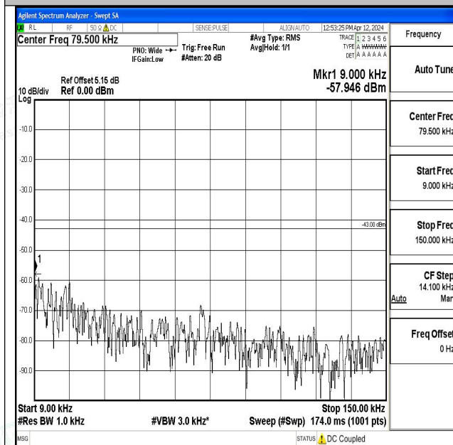
Band2_15MHz_QPSK_18900_1RB#0_0.009~0.15_0.009 ~0.15
