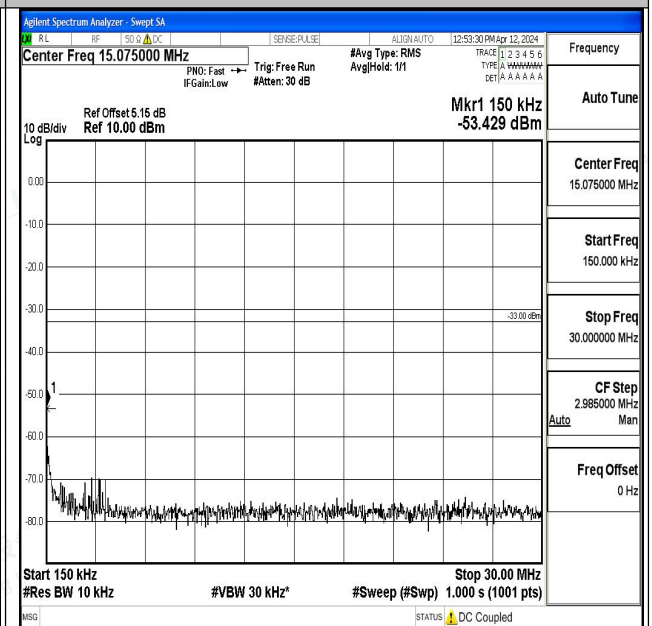
Band2_15MHz_QPSK_18900_1RB#0_0.15~30_0.15~30
