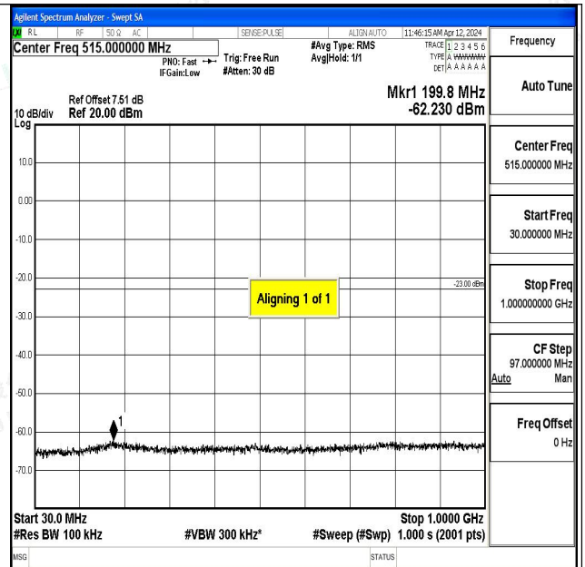
Band2_3MHz_16QAM_18615_1RB#0_30~1000_30~100
