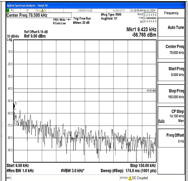
Band2_1.4MHz_16QAM_19193_1RB#0_0.009~0.15_0.09~0.15
