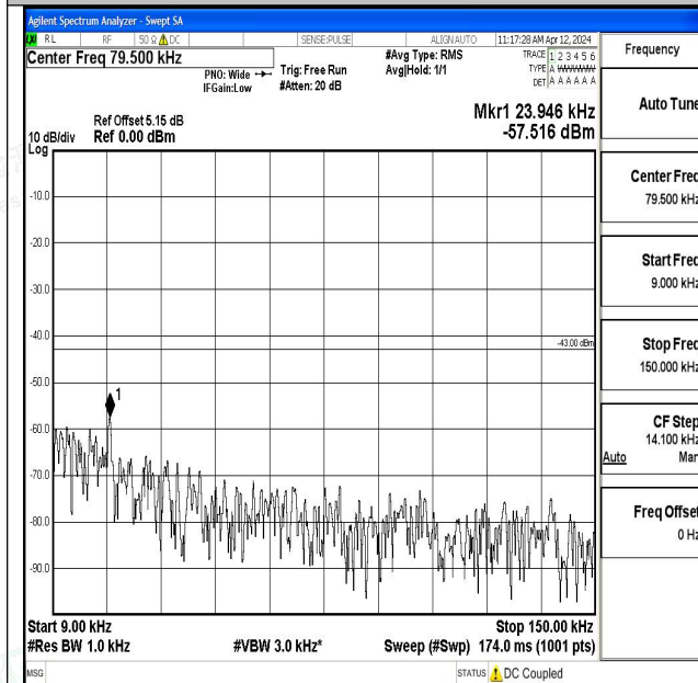
Band2_1.4MHz_QPSK_18900_1RB#0_0.009~0.15_0.00 9~0.15
