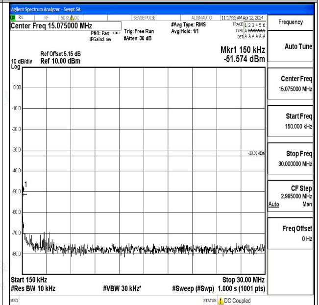
Band2_1.4MHz_QPSK_18900_1RB#0_0.15~30_0.15~30
