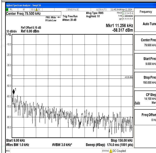
Band2_3MHz_QPSK_18615_1RB#0_0.009~0.15_0.009~ 0.15
