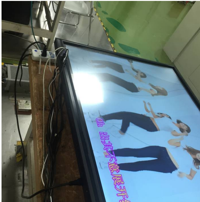
Conducted Emissions - Side View
