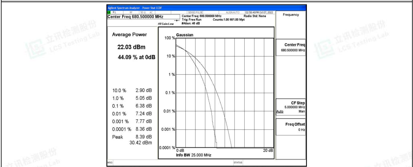
Band71-20MHz-16QAM-133372-100RB#0
