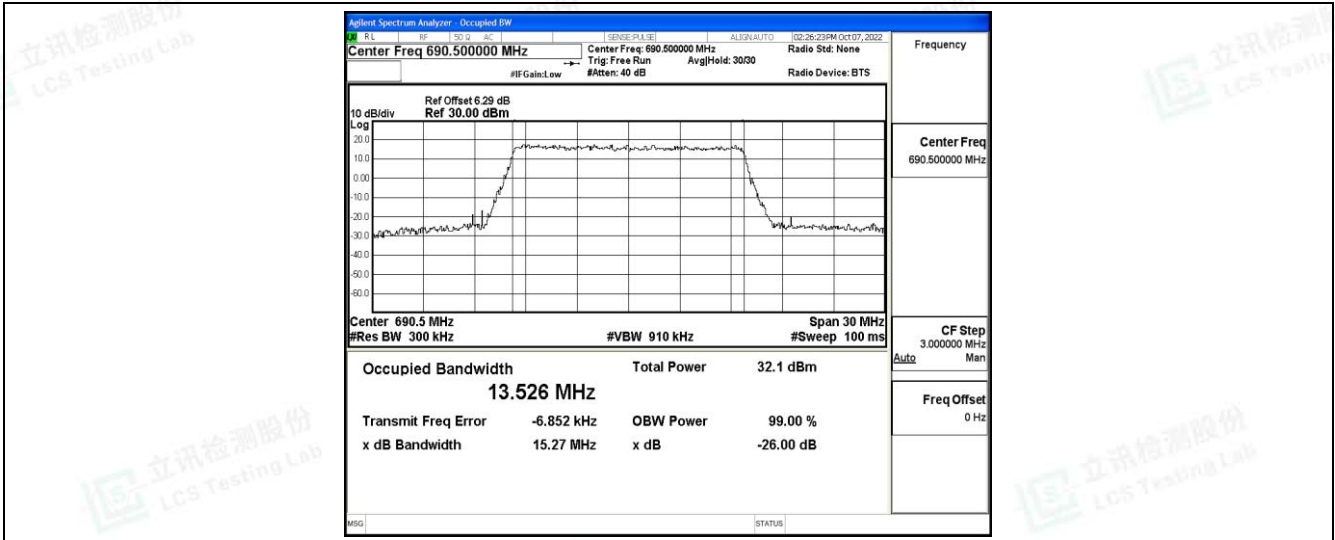
Band71-15MHz-16QAM-133197-75RB#0
