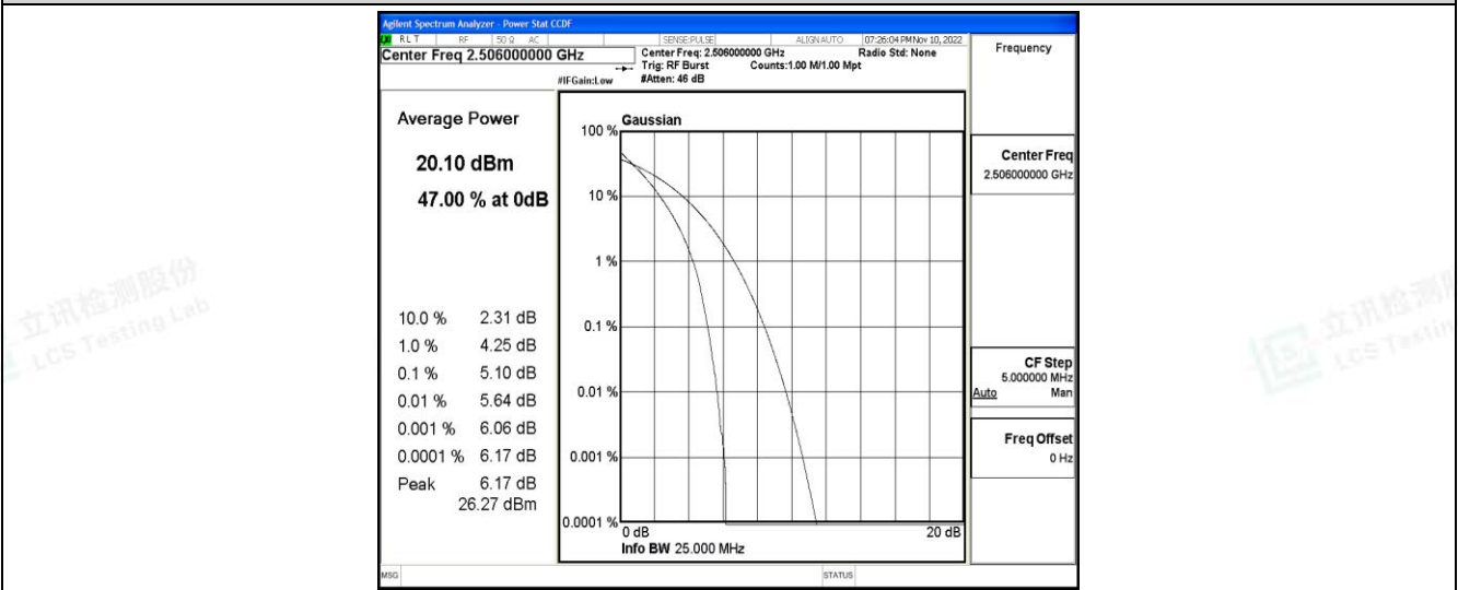
Band41-20MHz-QPSK-40620-100RB#0
