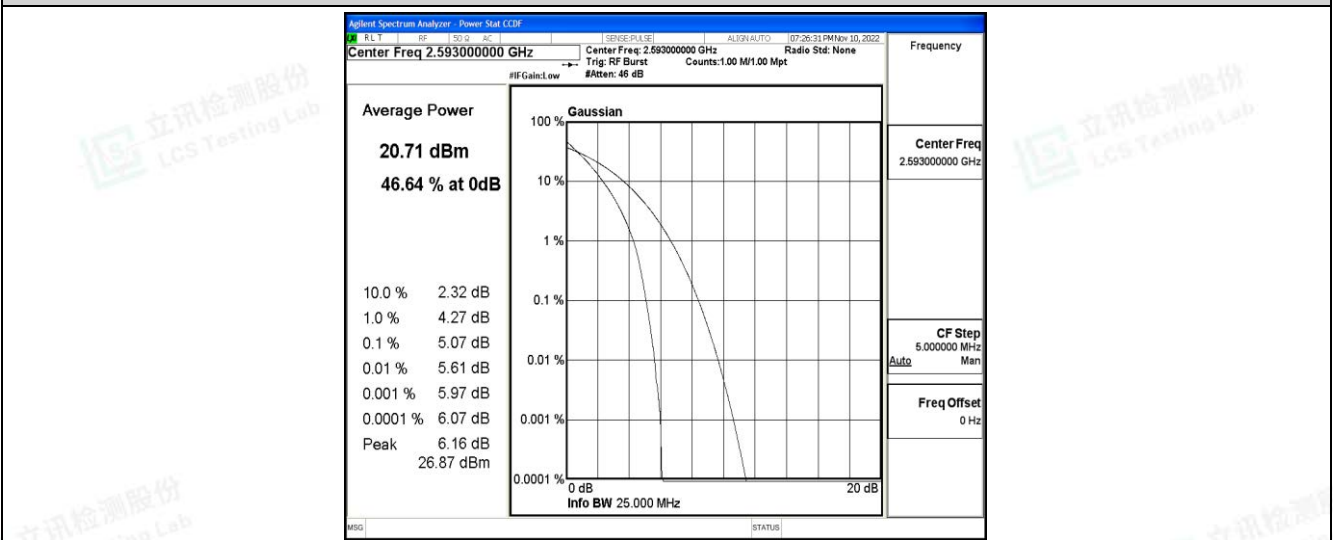
Band41-20MHz-QPSK-41490-100RB#0
