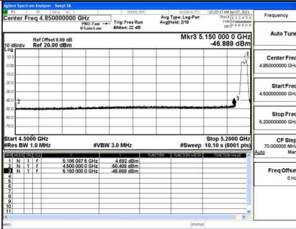
IEEE 802.11n20 / Channel 36 / 5180MHz / Peak
