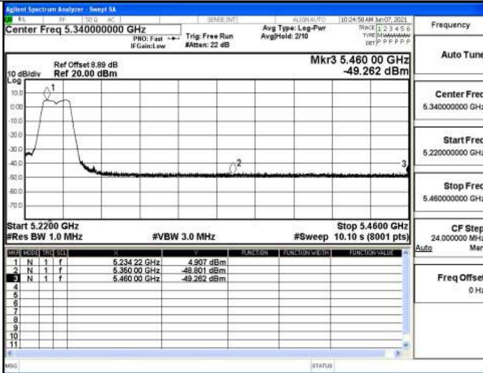
IEEE 802.11n20 / Channel 48 / 5240MHz / Peak
