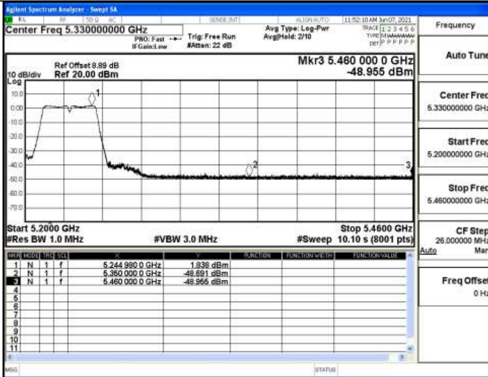
IEEE 802.11n40 / Channel 46 / 5230MHz / Peak
