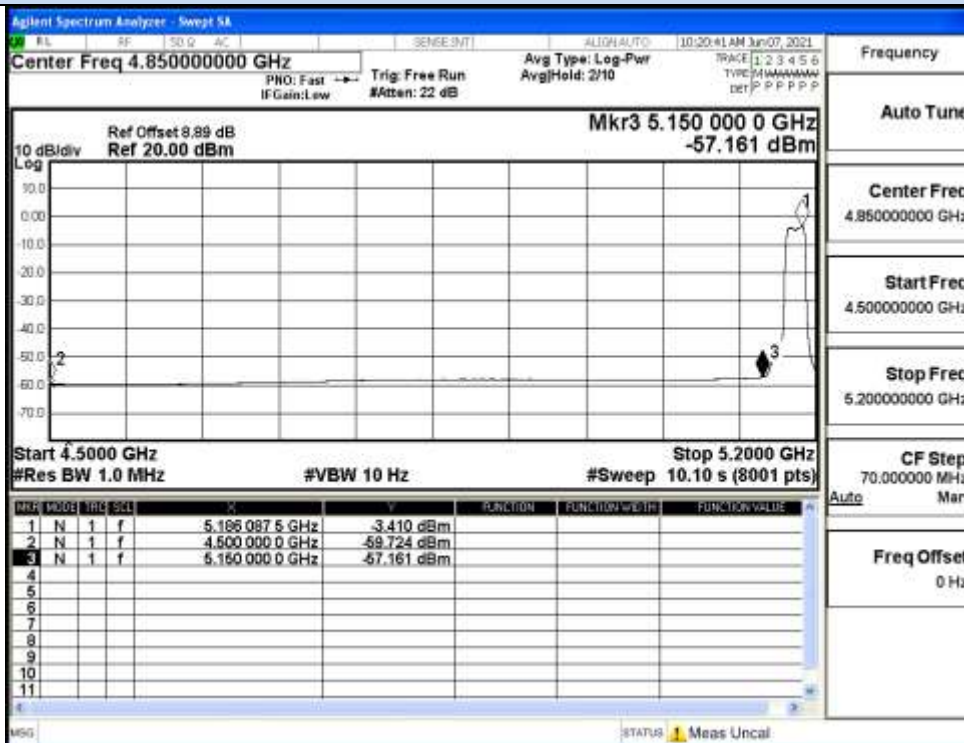
IEEE 802.11n20 / Channel 36 / 5180MHz / Average
