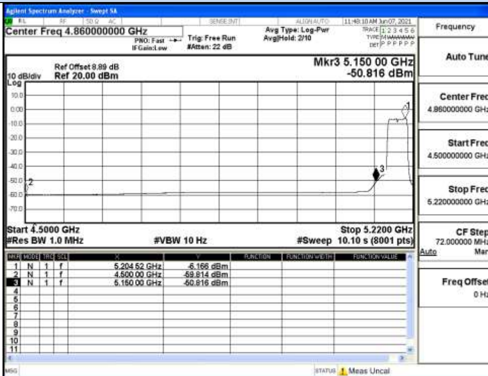
IEEE 802.11n40 / Channel 38 / 5190MHz / Average
