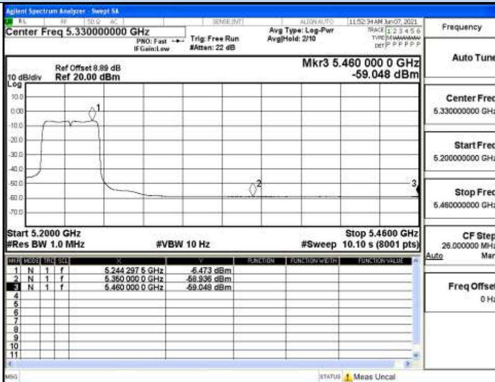
IEEE 802.11n40 / Channel 46 / 5230MHz / Average
