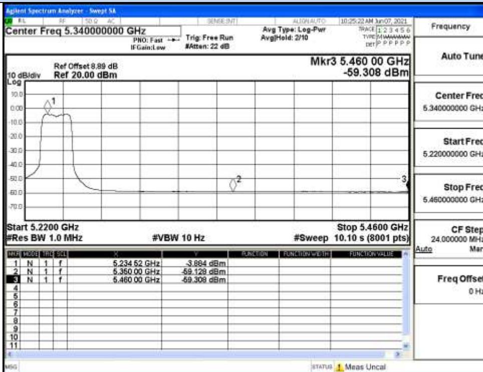
IEEE 802.11n20 / Channel 48 / 5240MHz / Average
