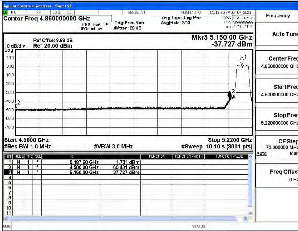
IEEE 802.11n40 / Channel 38 / 5190MHz / Peak
