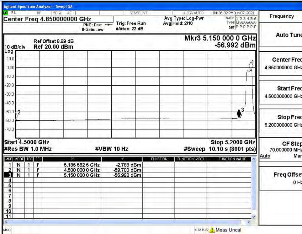
IEEE 802.11a / Channel 36 / 5180MHz / Average
