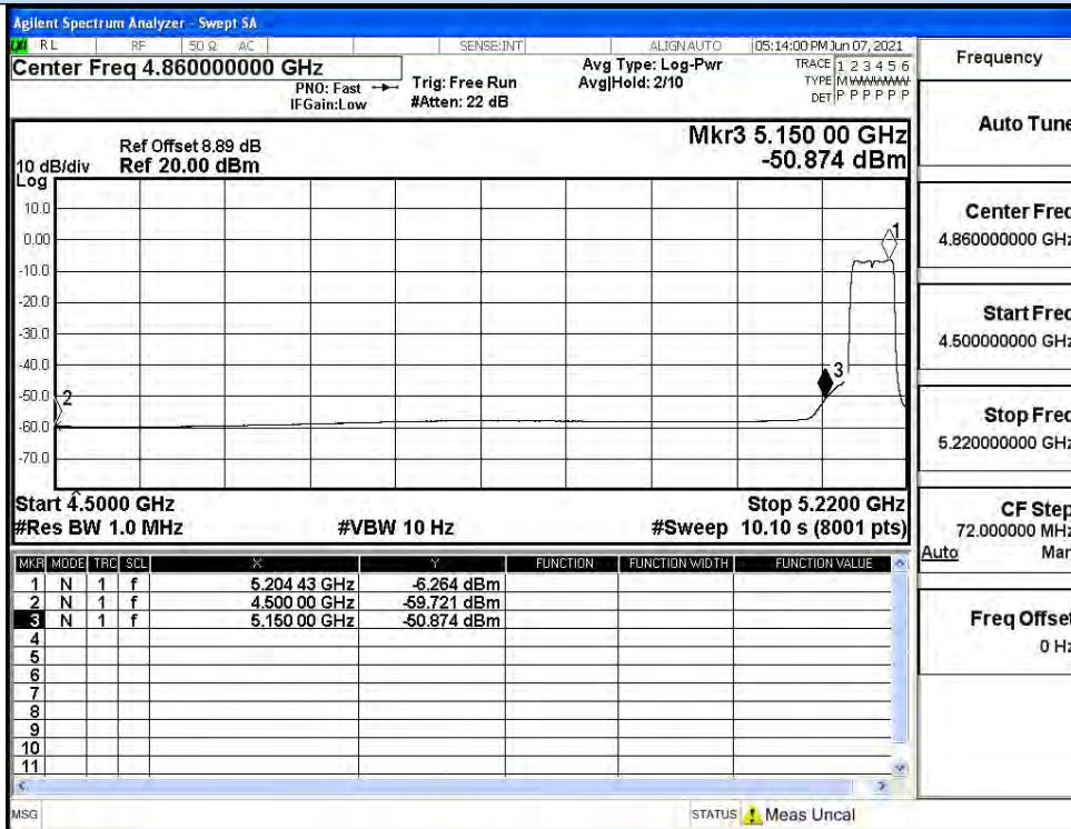
IEEE 802.11n40 / Channel 38 / 5190MHz / Average
