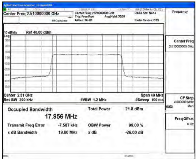
Band7-20MHz-16QAM-21100-100RB#0
