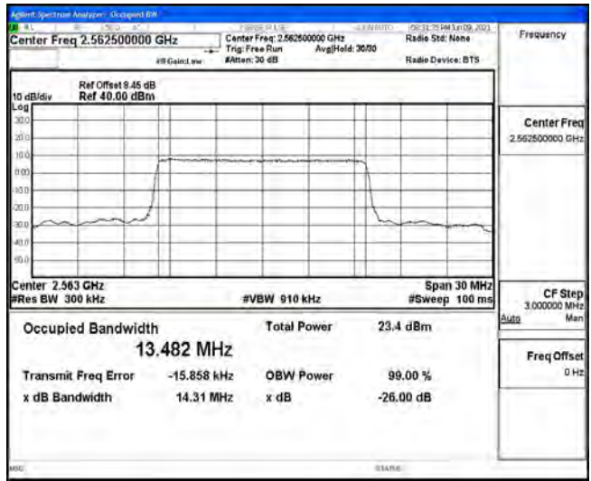
Band7-15MHz-16QAM-21375-75RB#0
