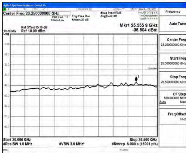
Band7-20MHz-16QAM-21350-1RB#0-Range6:20000~26500MHz
