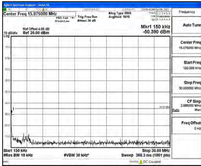
Band7-15MHz-QPSK-21100-1RB#0-Range3:30~1000MHz
