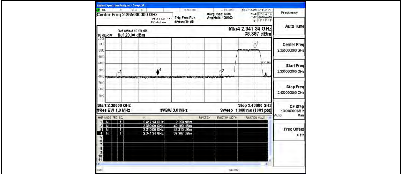
11N20SISO_Ant1_Low_2412_Peak
