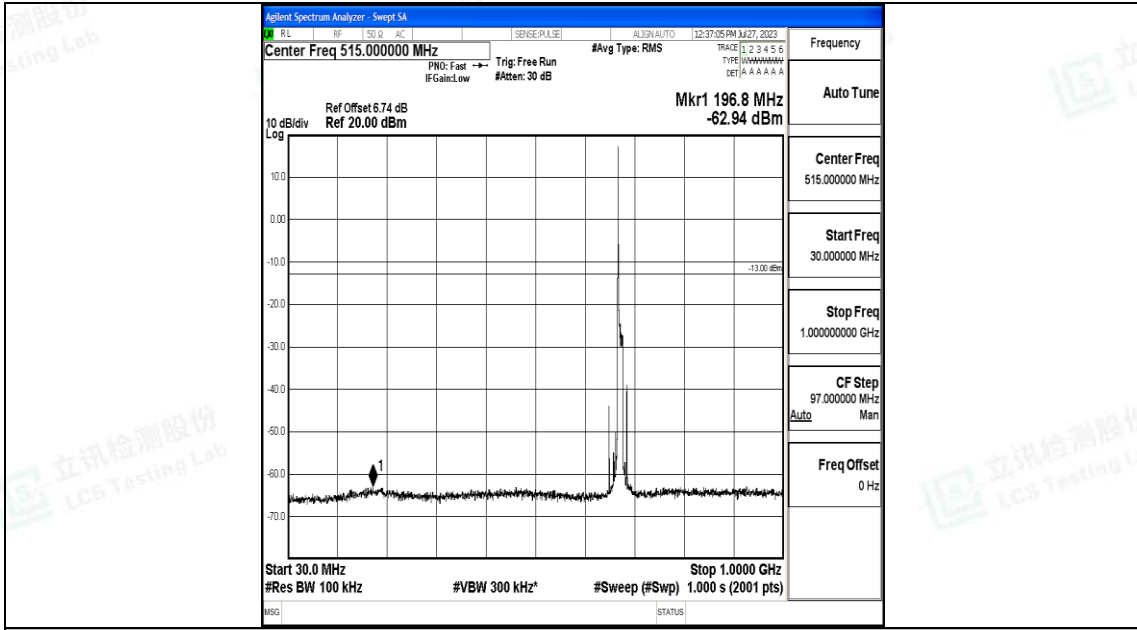
Band71_10MHz_QPSK_133297_1RB#0_30~1000_30~1000
