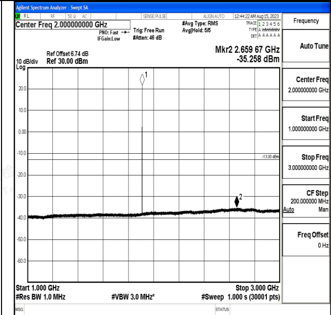
1 GHz – 3 GHz
