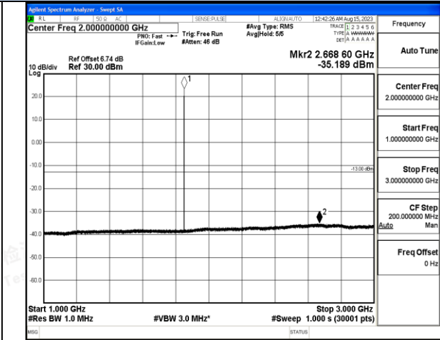
1 GHz – 3 GHz
