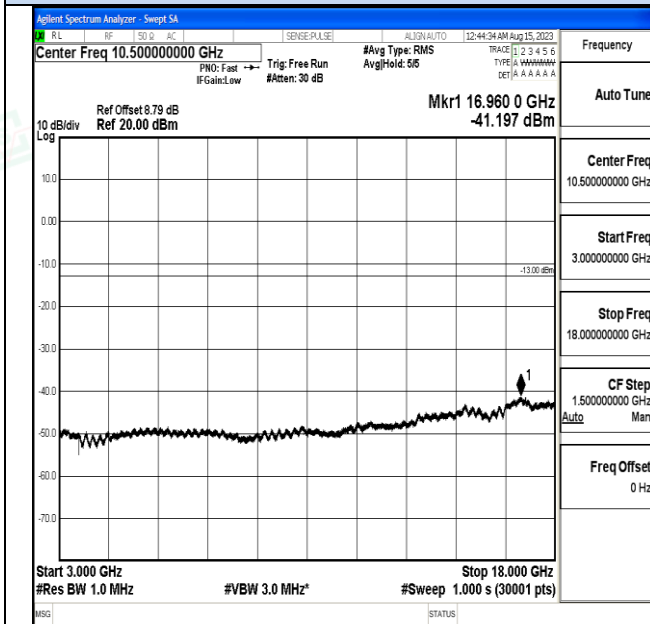
3 GHz – 18 GHz
