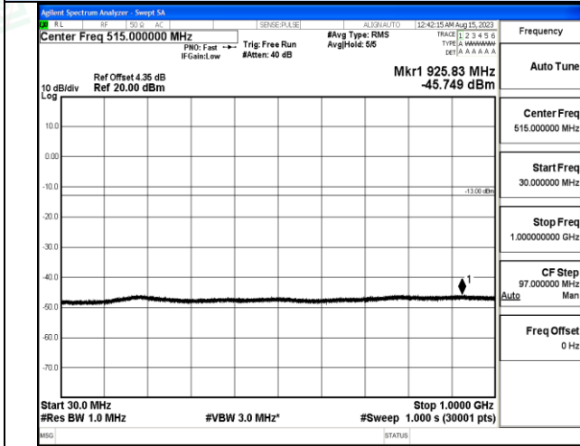
30 MHz – 1000 MHz
