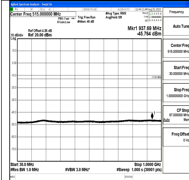
30 MHz – 1000 MHz
