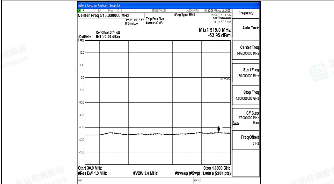
Band2_15MHz_16QAM_19125_1RB#0_30~1000_30~1000
