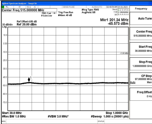
30 MHz – 1000 MHz
