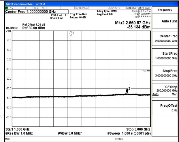
1 GHz – 3 GHz
