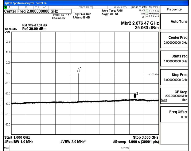
1 GHz – 3 GHz
