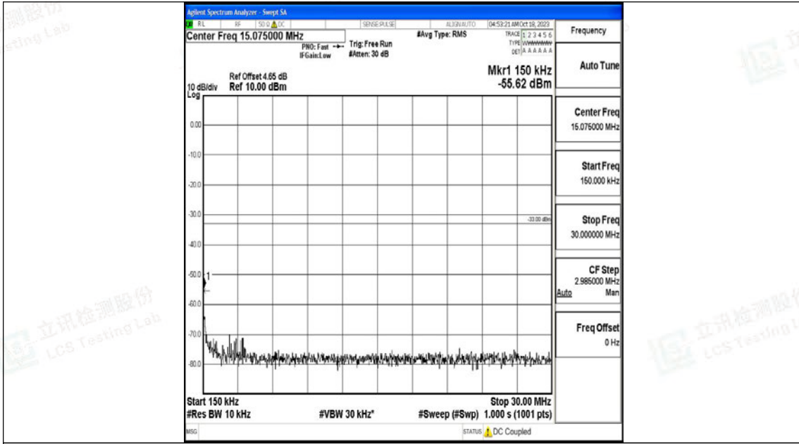
Band2_15MHz_16QAM_18900_1RB#0_0.15~30_0.15~30
