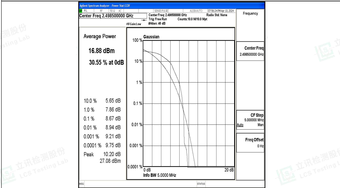
Band41-5MHz-16QAM-39675-1RB#0-PASS
