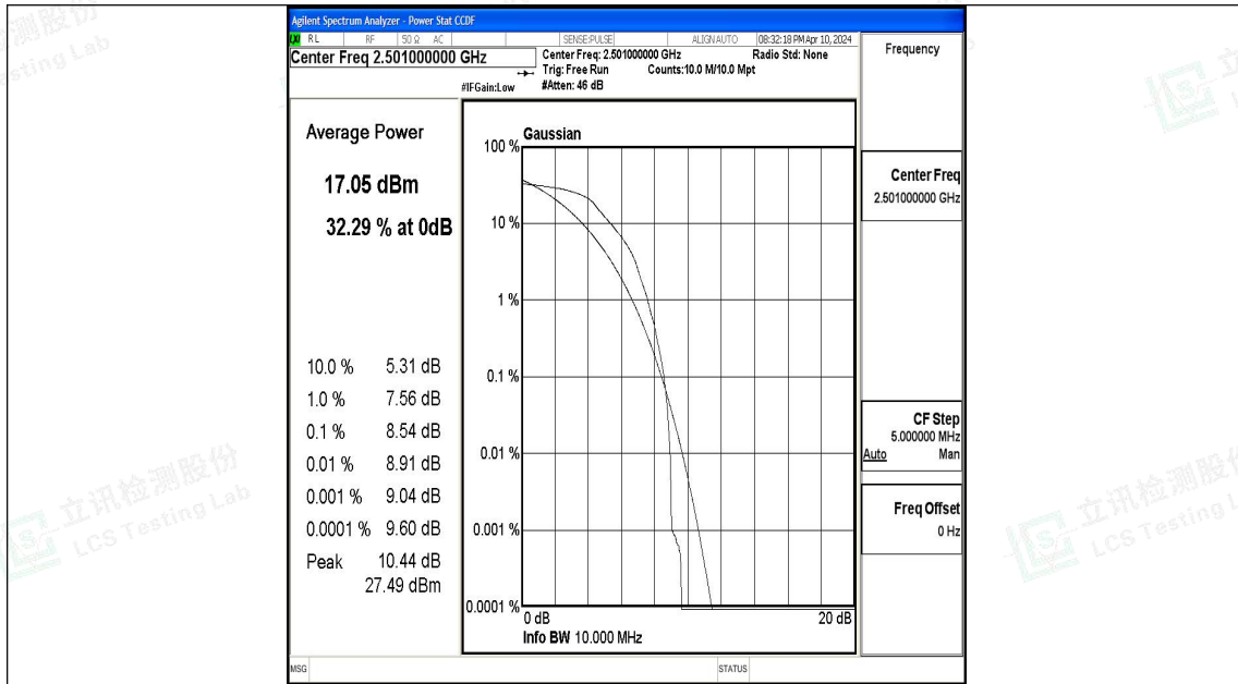
Band41-10MHz-QPSK-39700-1RB#0-PASS
