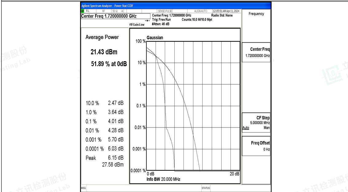
Band66-20MHz-16QAM-132072-1RB#0-PASS
