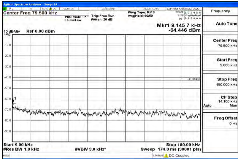
Band66-5MHz-QPSK-132322-1RB#0-Range2:0.15~30MHz
