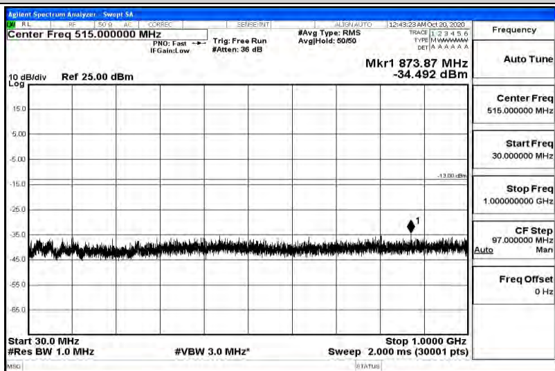
Band66-5MHz-16QAM-131997-1RB#0-Range4:1000~5000MHz
