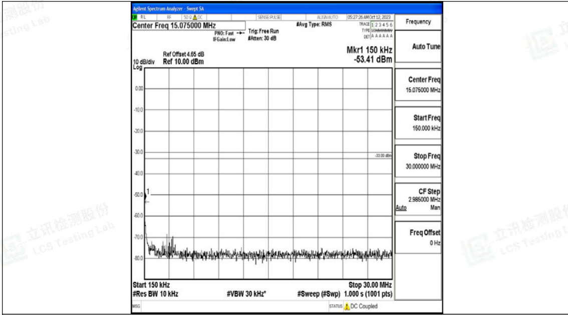
Band4_10MHz_16QAM_20350_1RB#0_0.15~30_0.15~30
