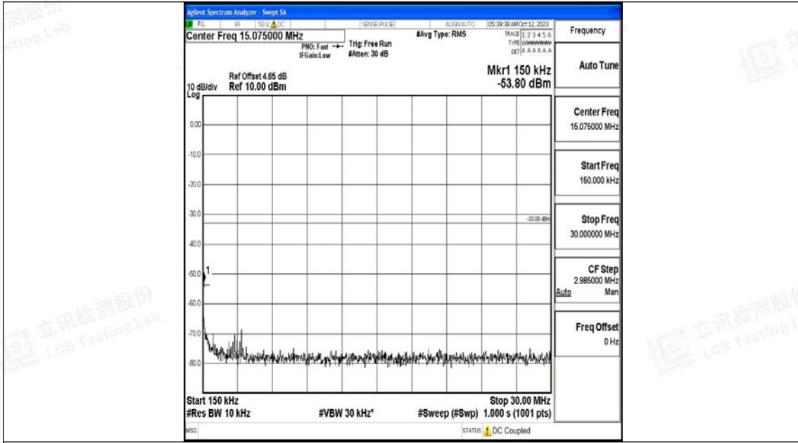
Band4_15MHz_16QAM_2025_1RB#0_0.15~30_0.15~30
