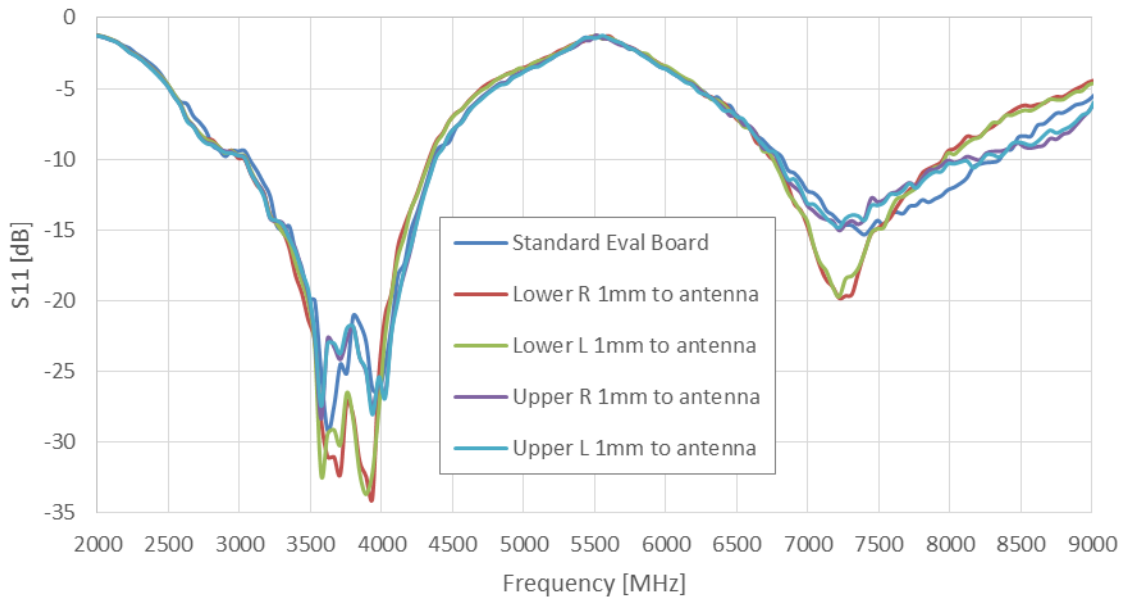
Return loss for clearance study (metal component next to antenna)
