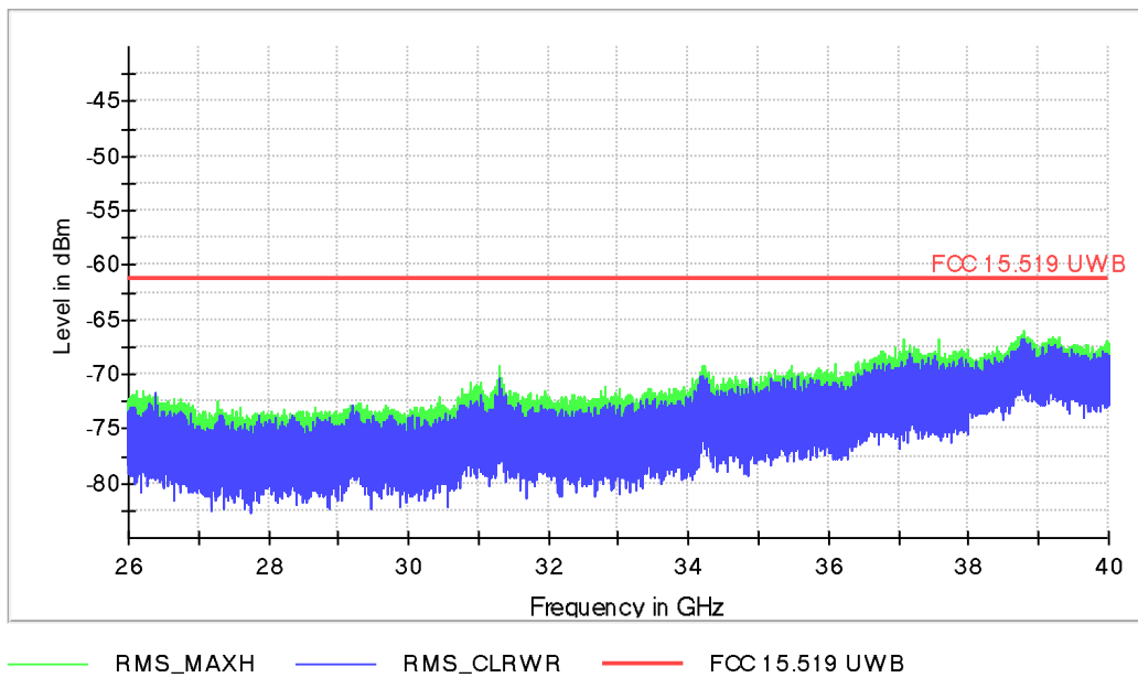
FCC 15.519_26GHz-40GHz
