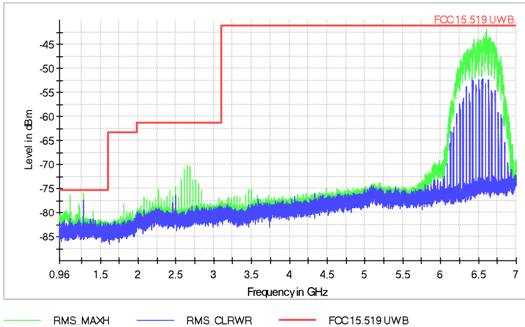
FCC15.519_960MHz-7GHz
