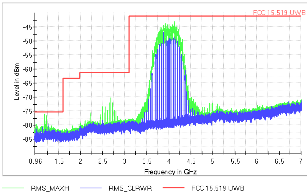
FCC 15.519_960MHz-7GHz
