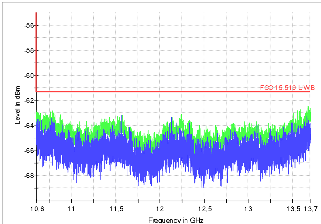
FCC 15.519_10.6-13.7GHz
