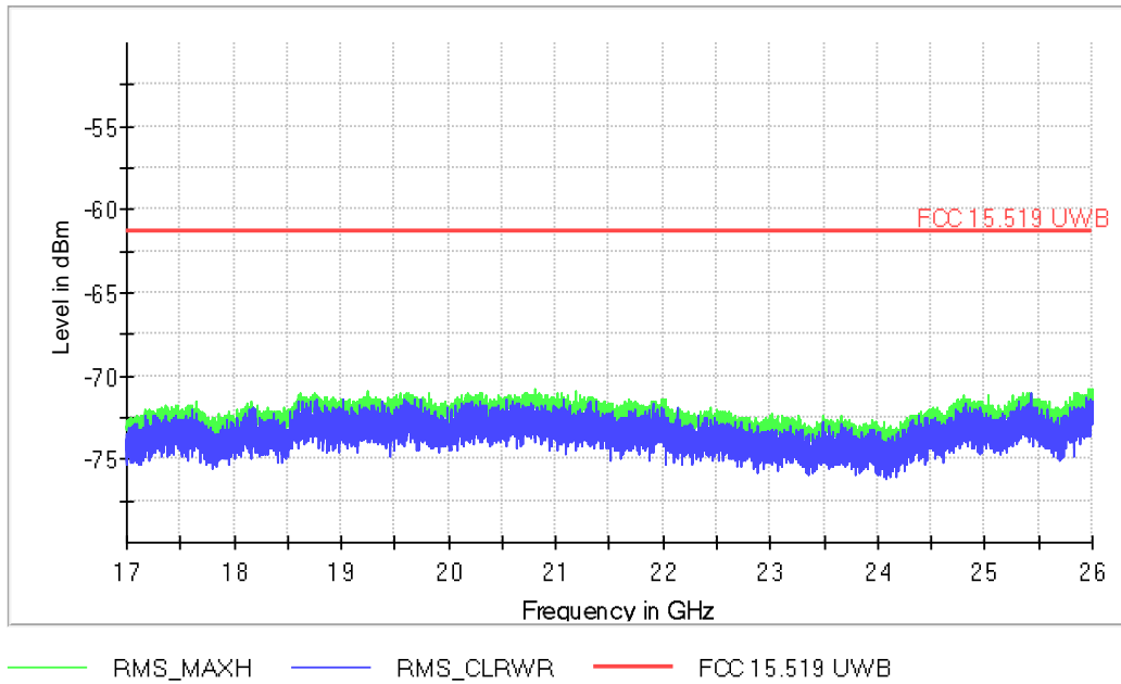
FCC 15.519_17GHz-26GHz
