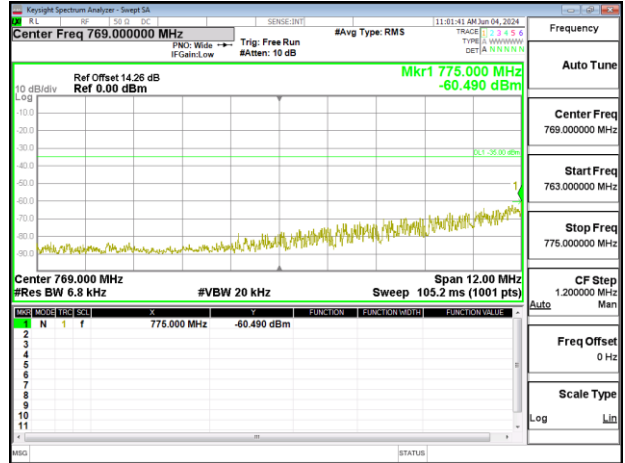
Band13_10MHz_QPSK_RB6_0_CH23230_index7
