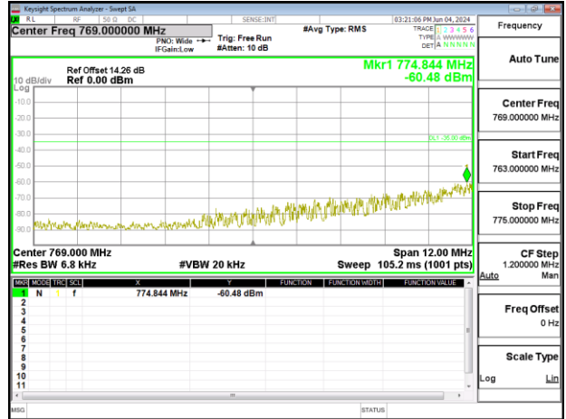
Band13_5MHz_QPSK_RB6_0_CH23255
