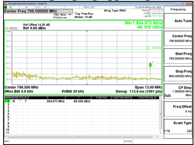
Band13_10MHz_QPSK_RB6_0_CH23230_index7
