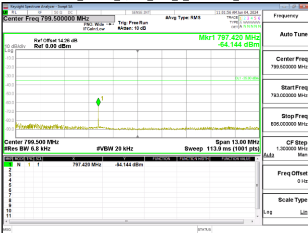
Band13_10MHz_QPSK_RB6_0_CH23230_index0
