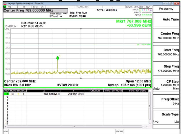
Band13_5MHz_QPSK_RB6_0_CH23205
