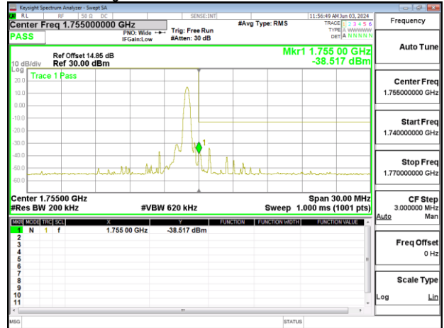
Band Edge_Band4_15MHz_QPSK_RB1_5_CH20325
