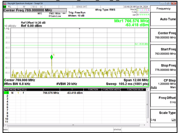
Band13_10MHz_QPSK_RB6_0_CH23230_index0
