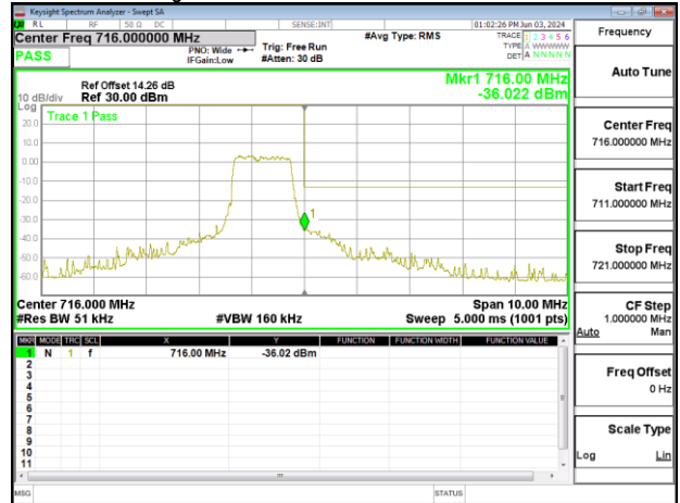
Band Edge_Band12_5MHz_QPSK_RB6_0_CH2155
