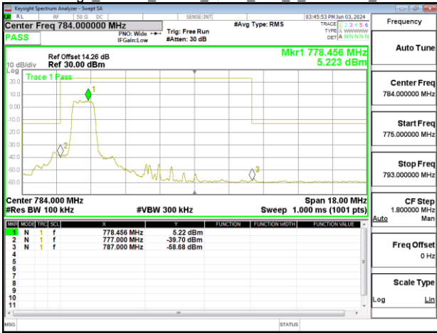
Band Edge_Band13_10MHz_QPSK_RB6_0_CH23230_index7
