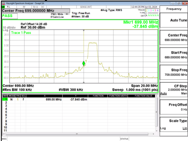
Band Edge_Band12_10MHz_QPSK_RB6_0_CH23060
