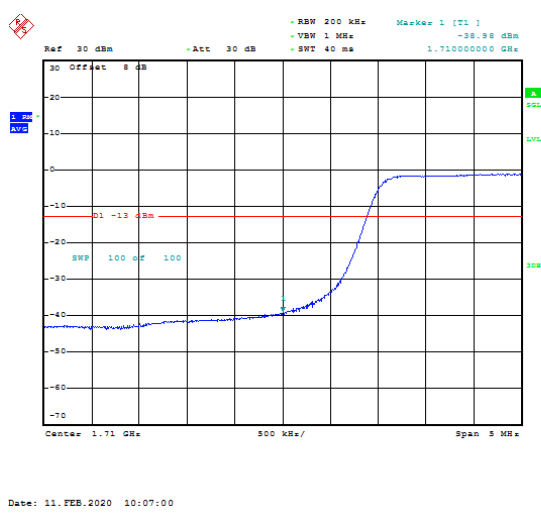
LOW BAND EDGE BLOCK-20MHz-100%RB
