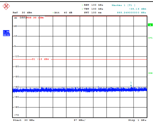
Channel 1512: 30MHz~1GHz
