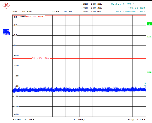
Channel 1312: 30MHz~1GHz
