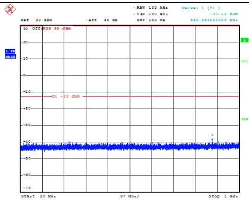
Channel 1450: 30MHz~1GHz
