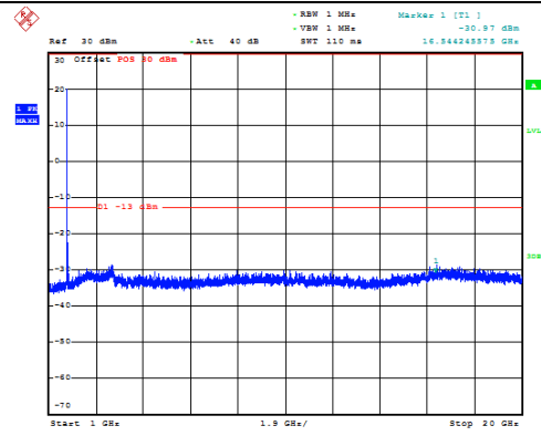
Channel 1312: 1GHz~20GHz
