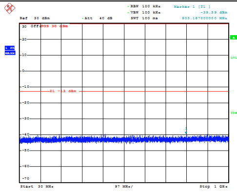
Channel 9262: 30MHz~1GHz
