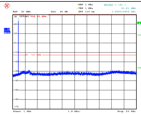
Channel 9538: 1GHz~20GHz
