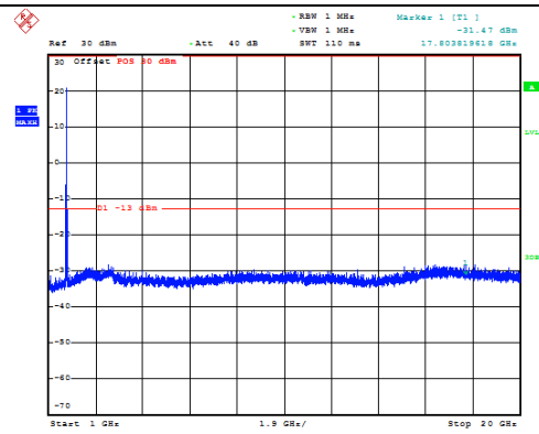
Channel 1450: 1GHz~20GHz
