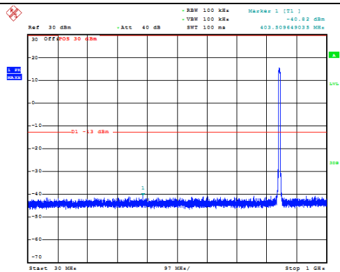
Channel 4175: 30MHz~1GHz
