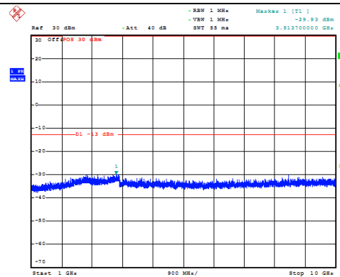
Channel 4175: 1GHz~10GHz
