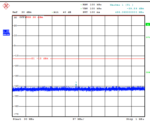
Channel 9400: 30MHz~1GHz
