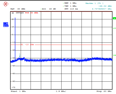
Channel 9262: 1GHz~20GHz
