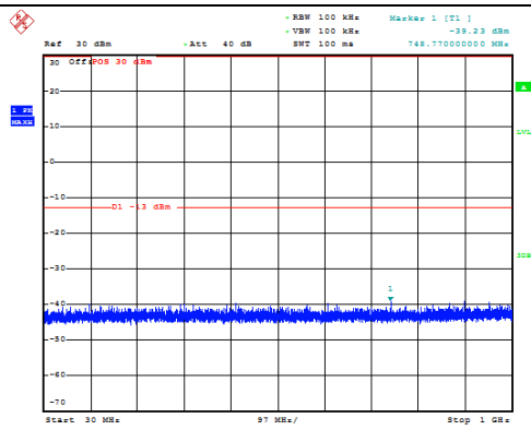
Channel 9538: 30MHz~1GHz
