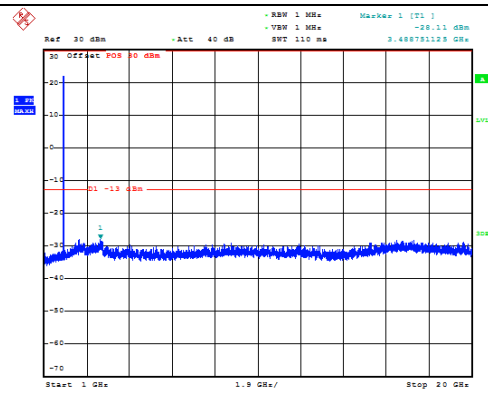
Channel 9400: 1GHz~20GHz
