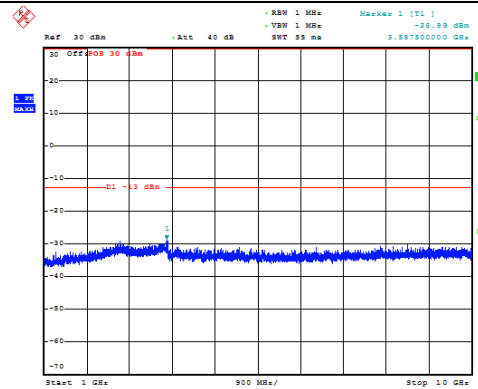
Channel 4133: 1GHz~10GHz
