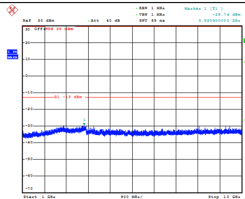
Channel 4232: 1GHz~10GHz
